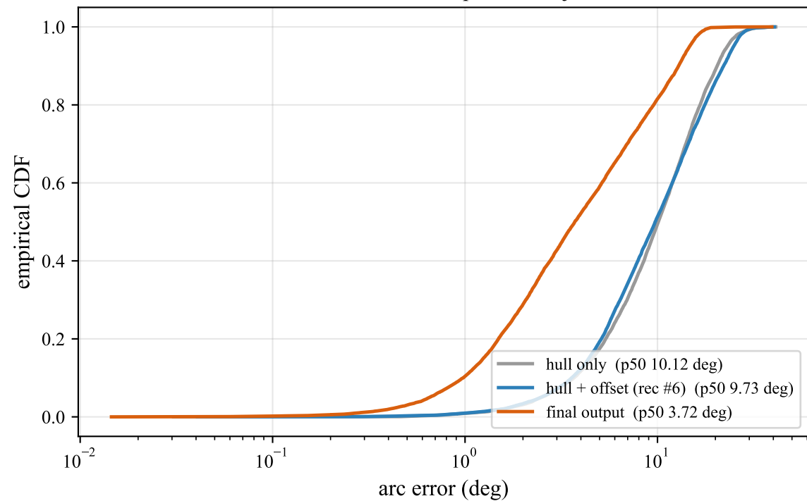
Phase 5: anchor decomposition, 1 jammer
