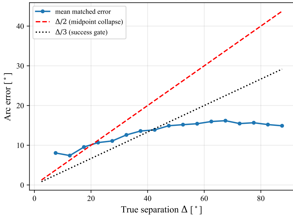
(b) Error against the collapse signature
