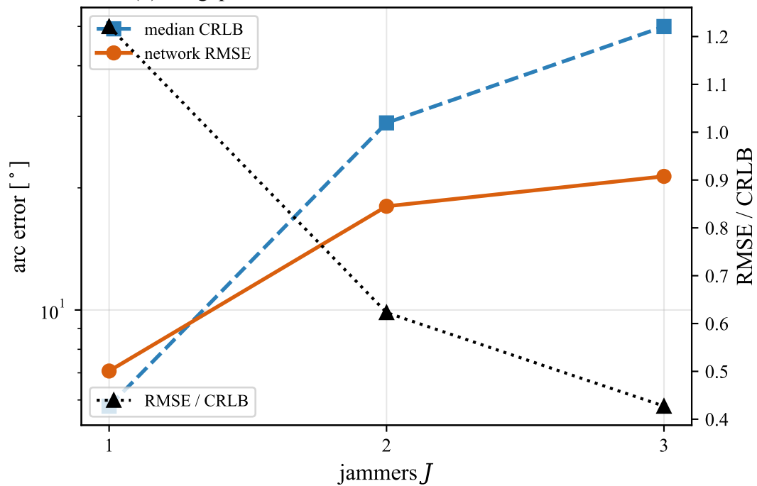
(d) the gap to the bound, not the network, is what closes
