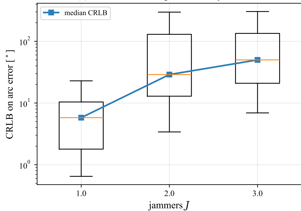
(c) the bound itself degrades, for any estimator
