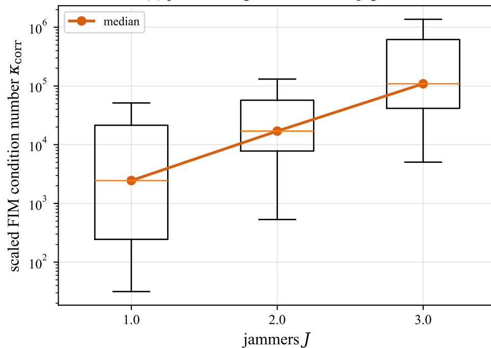
(b) parameters grow collinear as J grows
