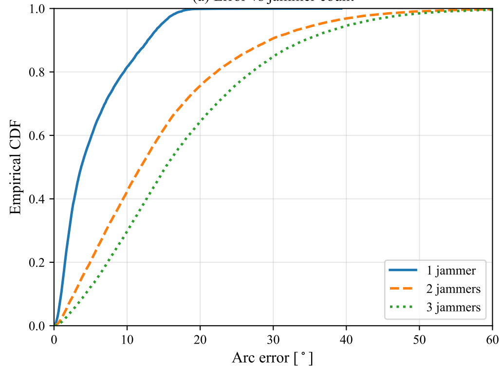
(a) Error vs jammer count
