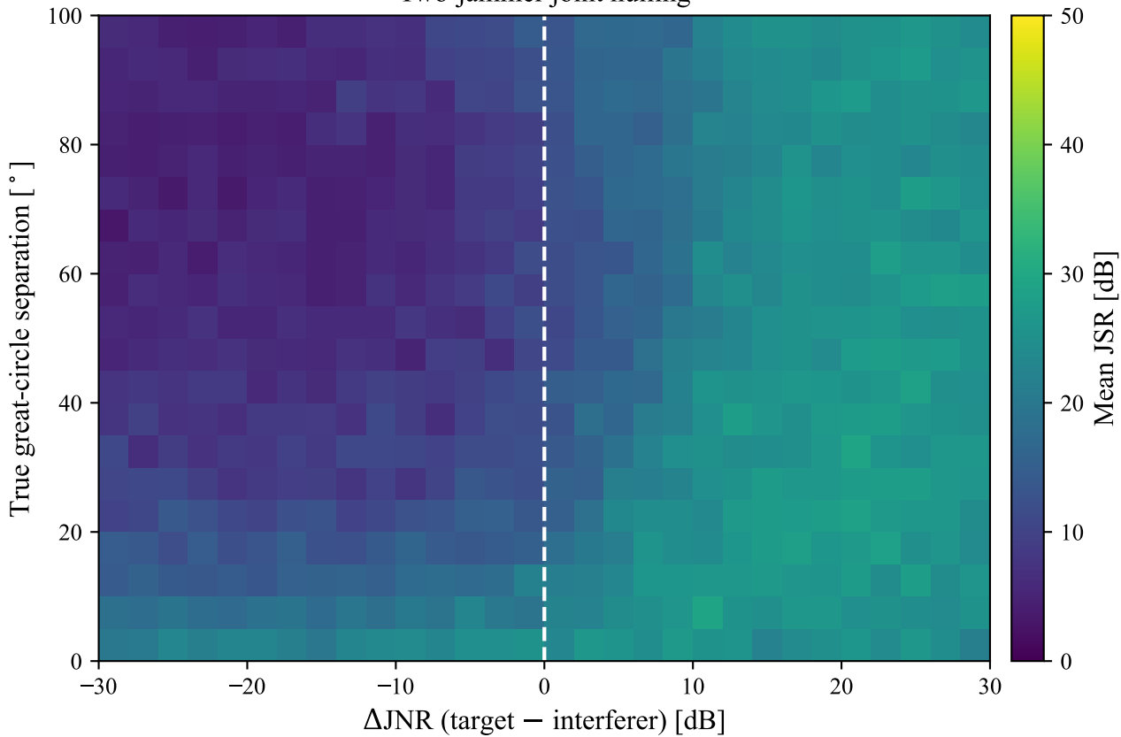
Two-jammer joint nulling
