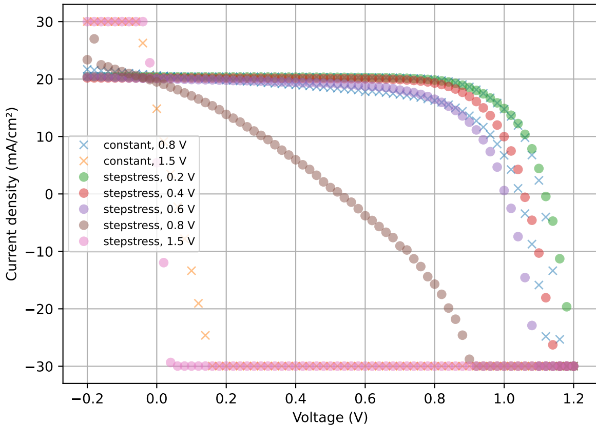
Type-1 JV by stress mode and voltage
