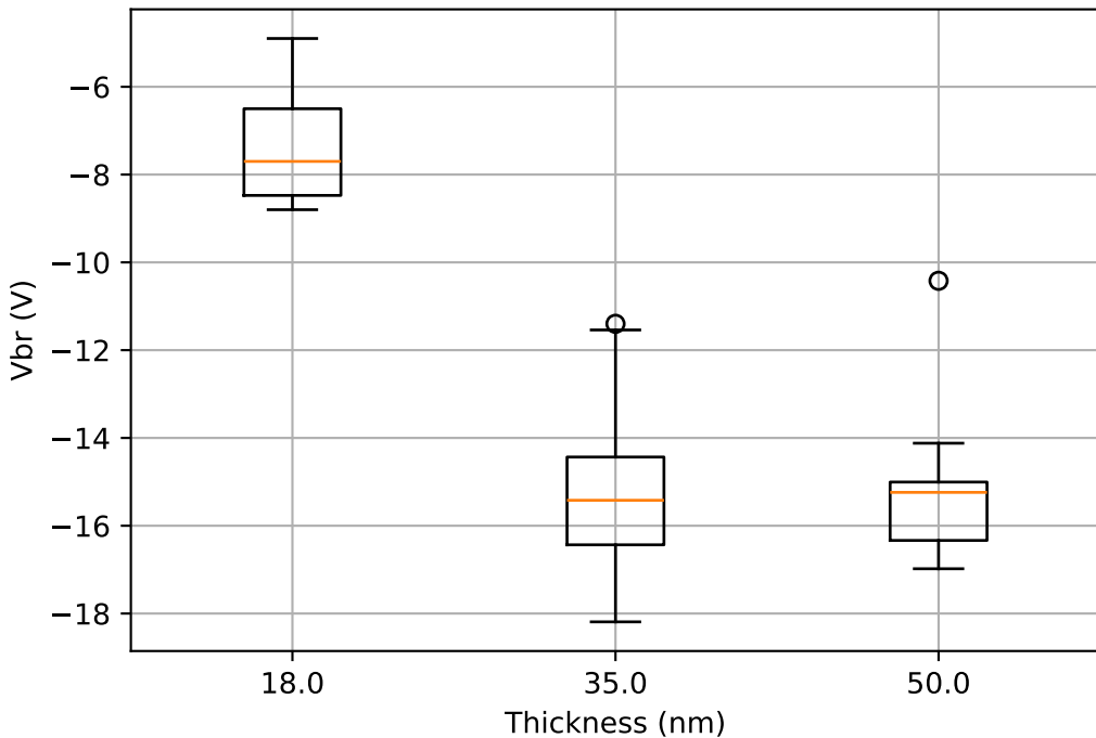
Type-4: Vbr by thickness — PTAA
