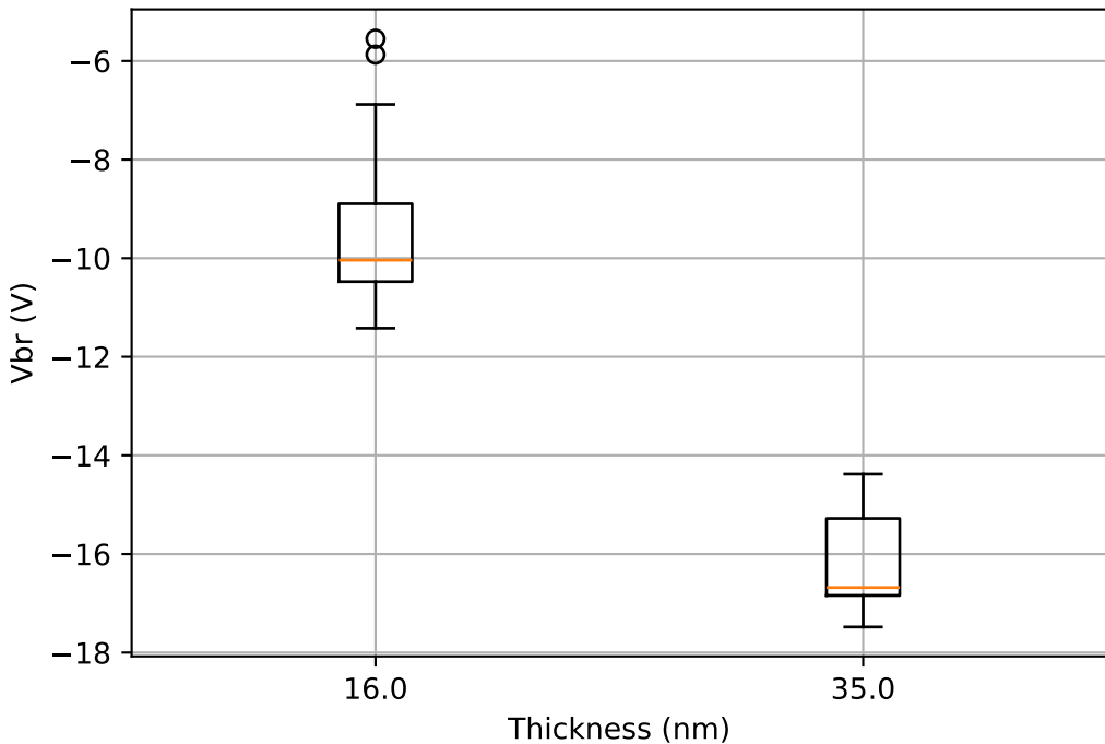
Type-4: V br by thickness — Poly-TPD
