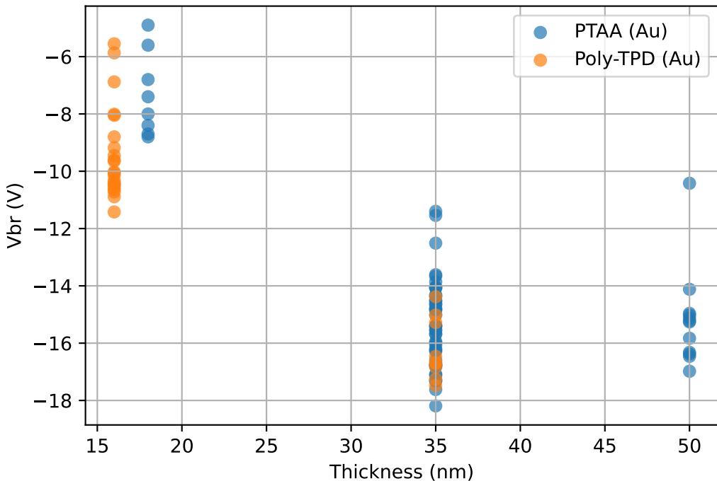
Type-4: Breakdown voltage vs HTL thickness
