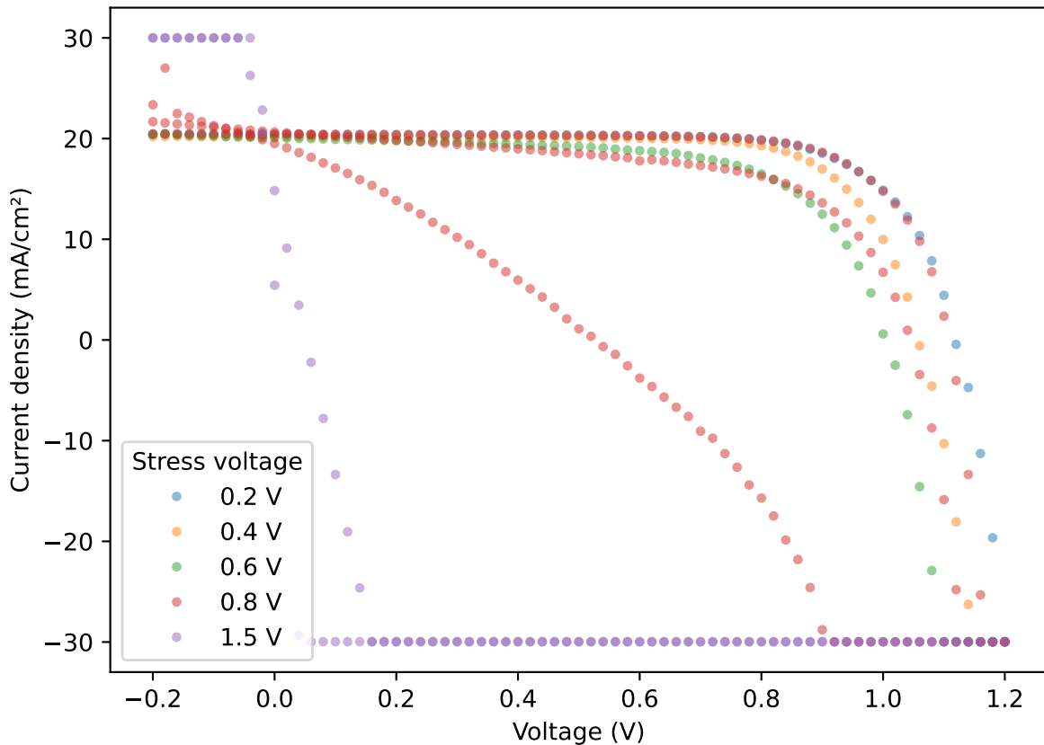
Type-1 JV curves by stress voltage
