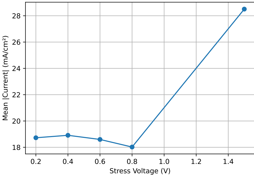
Leakage current vs stress voltage
