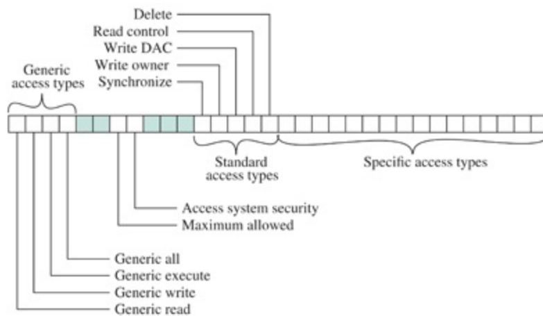
Figure 15.10 Access Mask
