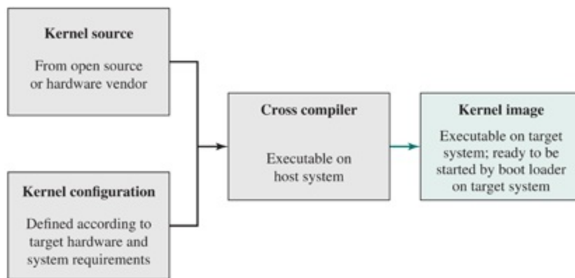
Figure 13.5 Kernel Compilation
