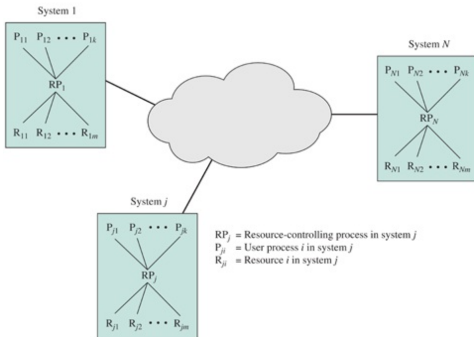
Figure 19.7 Model for Mutual Exclusion Problem in Distributed
