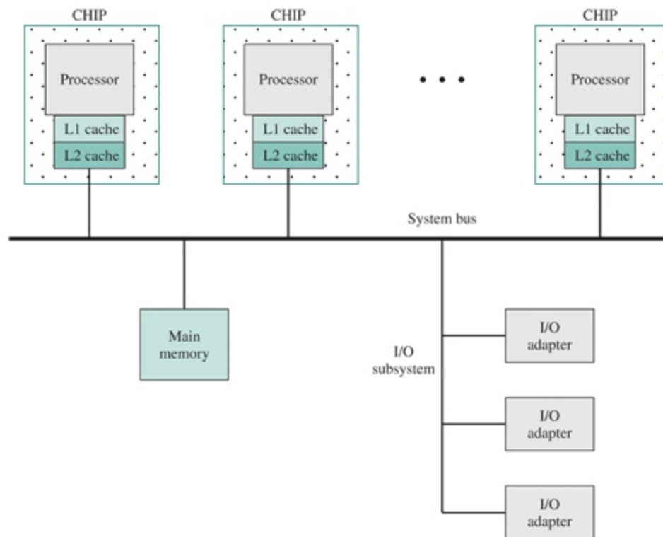
Figure 1.19 Symmetric Multiprocessor Organization
