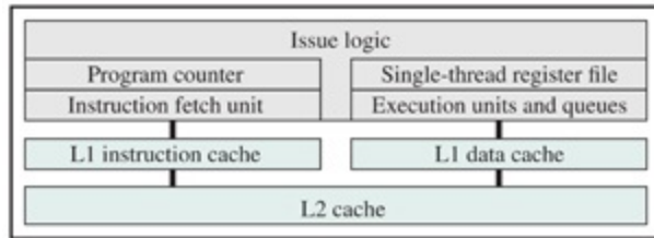
(a) Superscalar
