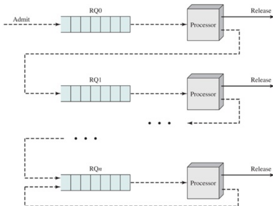
Figure 9.10 Feedback Scheduling
