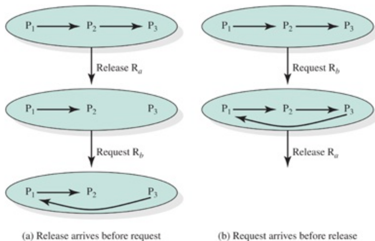
Figure 19.12 Phantom Deadlock
