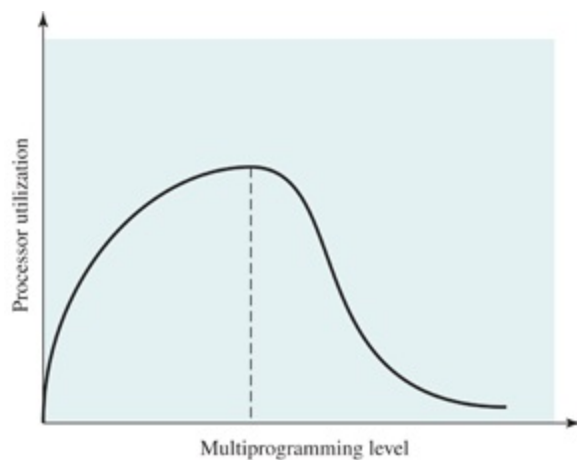
Figure 8.19 Multiprogramming Effects
