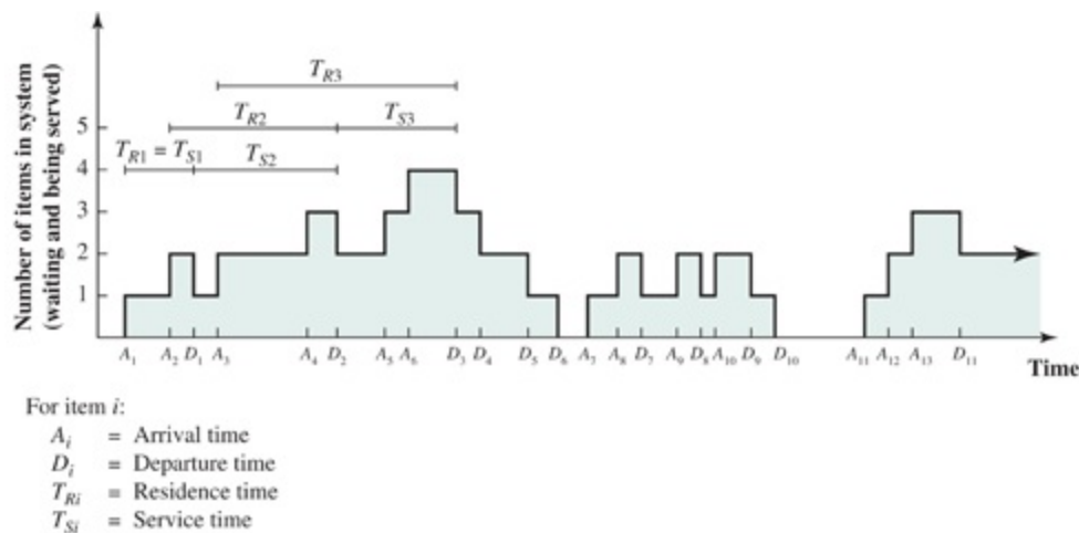
Figure 21.3 Example of a Queueing Process
