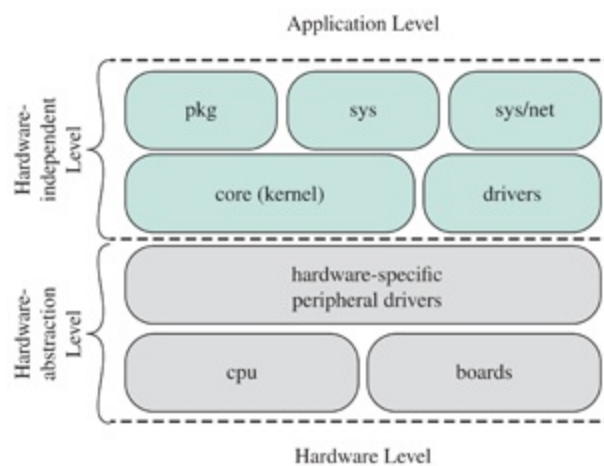
Figure 16.14 RIOT Structure
