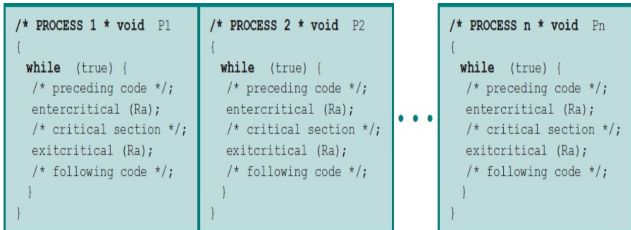
Figure 5.4 Illustration of Mutual Exclusion
