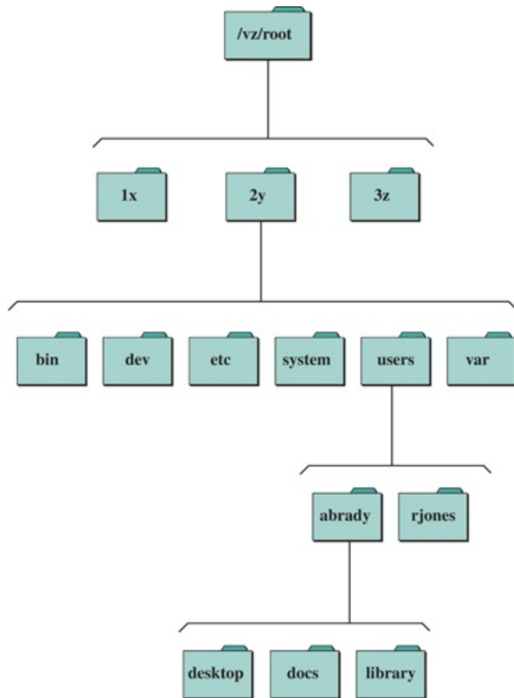
Figure 14.6 OpenVZ File scheme
