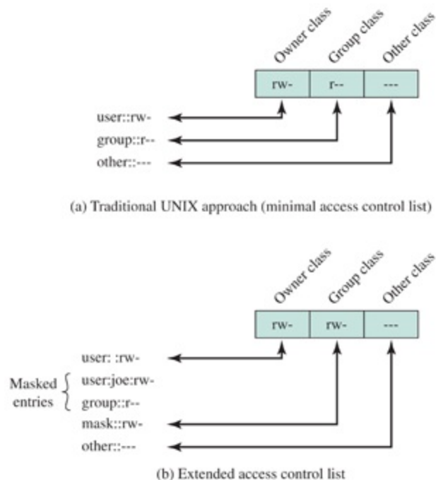
Figure 15.8 UNIX File Access Control
