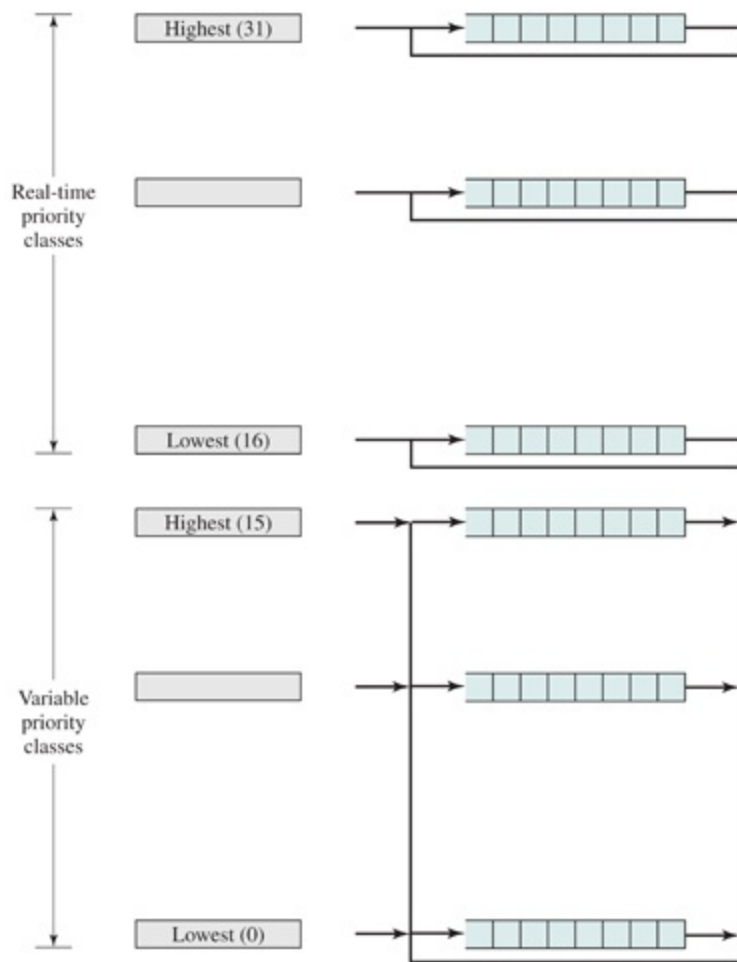
Figure 10.14 Windows Thread Dispatching Priorities
