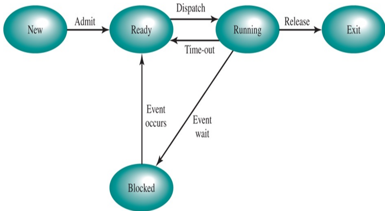
Figure 3.6 Five-State Process Model
