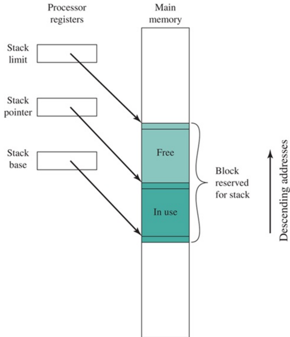
Figure P.1 Typical Stack Organization (full/descending)
