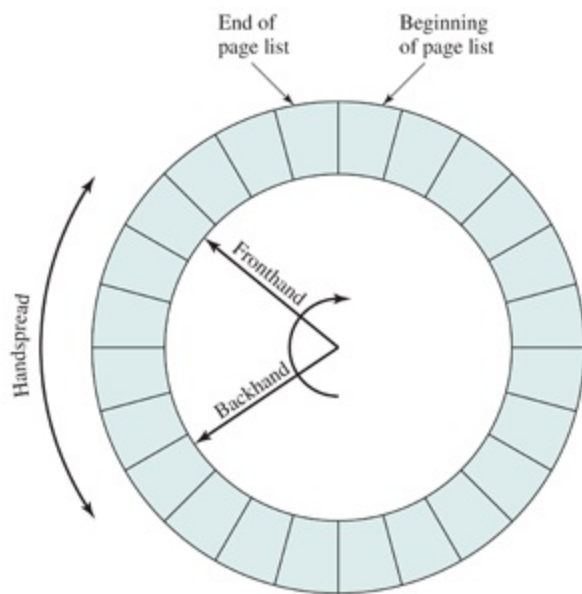
Figure 8.21 Two-Handed Clock Page Replacement Algorithm
