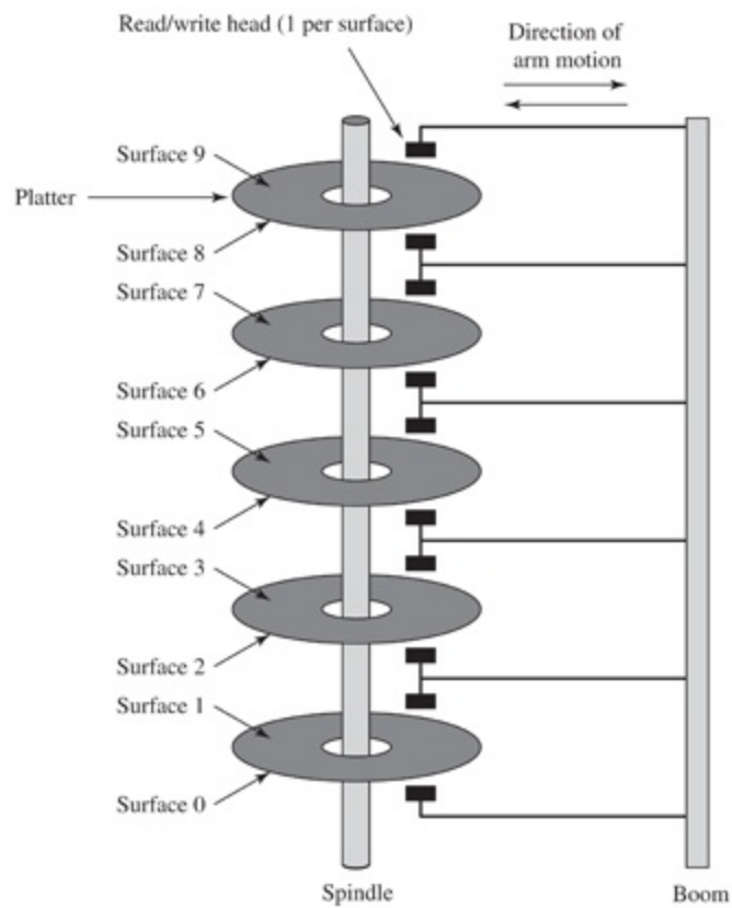
Figure J.4 Tracks and Cylinders
