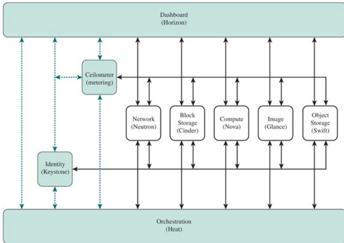
Figure 16.9 OpenStack High Level Architecture
