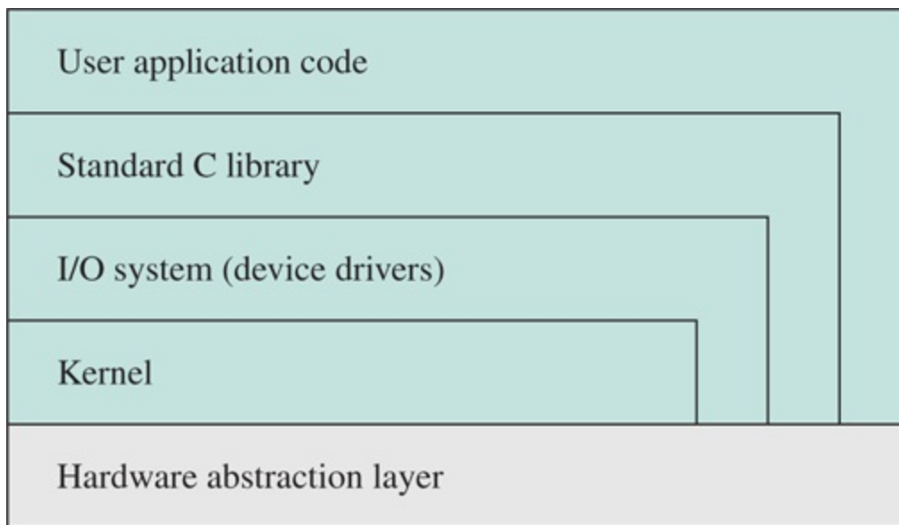
Figure Q.4 eCos Layered Structure
