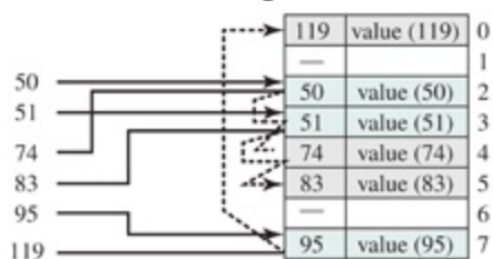
Figure F.1 Hashing
