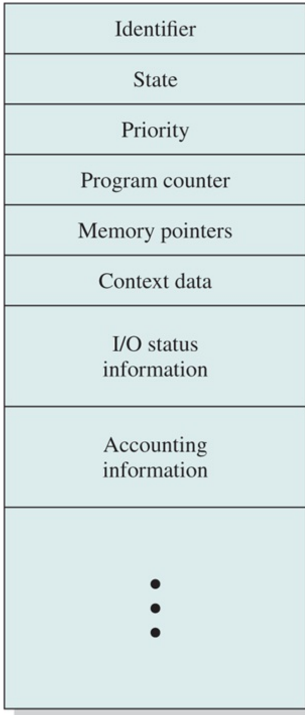
Figure 3.1 Simplified Process Control Block
