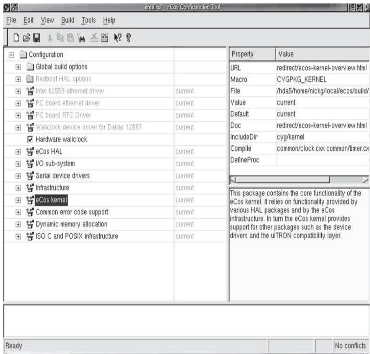
Figure Q.1 eCos Configuration Tool - Top Level
