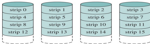
(a) RAID 0 (nonredundant)
