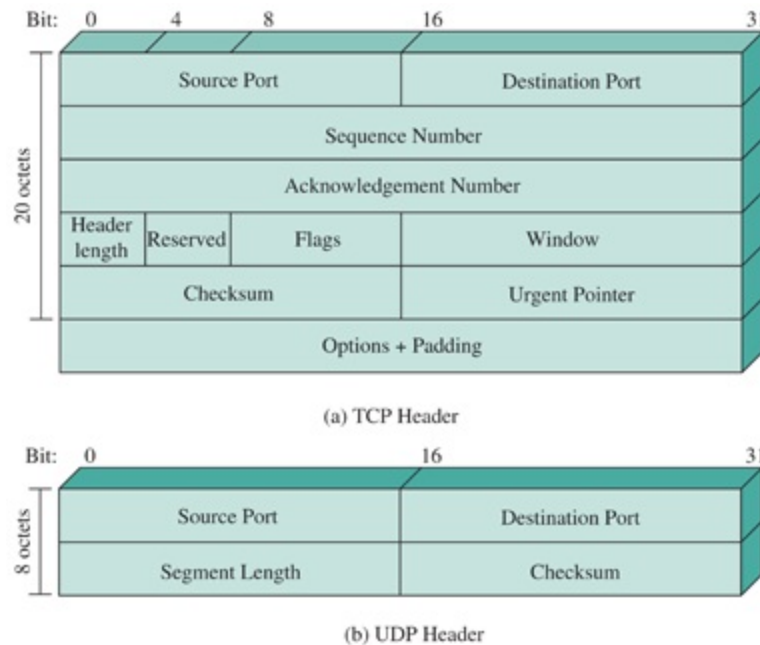
Figure 17.2 TCP and UDP Headers
