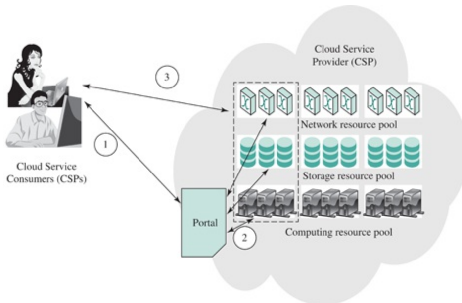
Figure 16.5 IaaS Conceptual Framework
