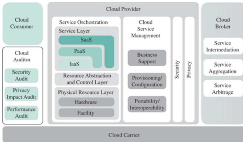
Figure 16.3 NIST Cloud Computing Reference Architecture
