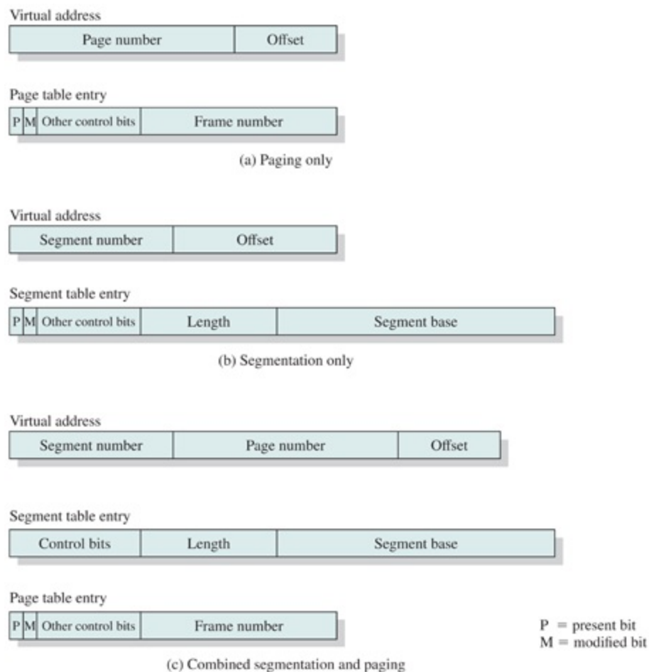
Figure 8.1 Typical Memory Management Formats
