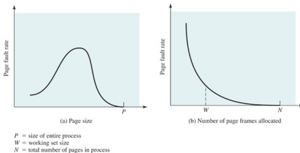
Figure 8.10 Typical Paging Behavior of a Program
