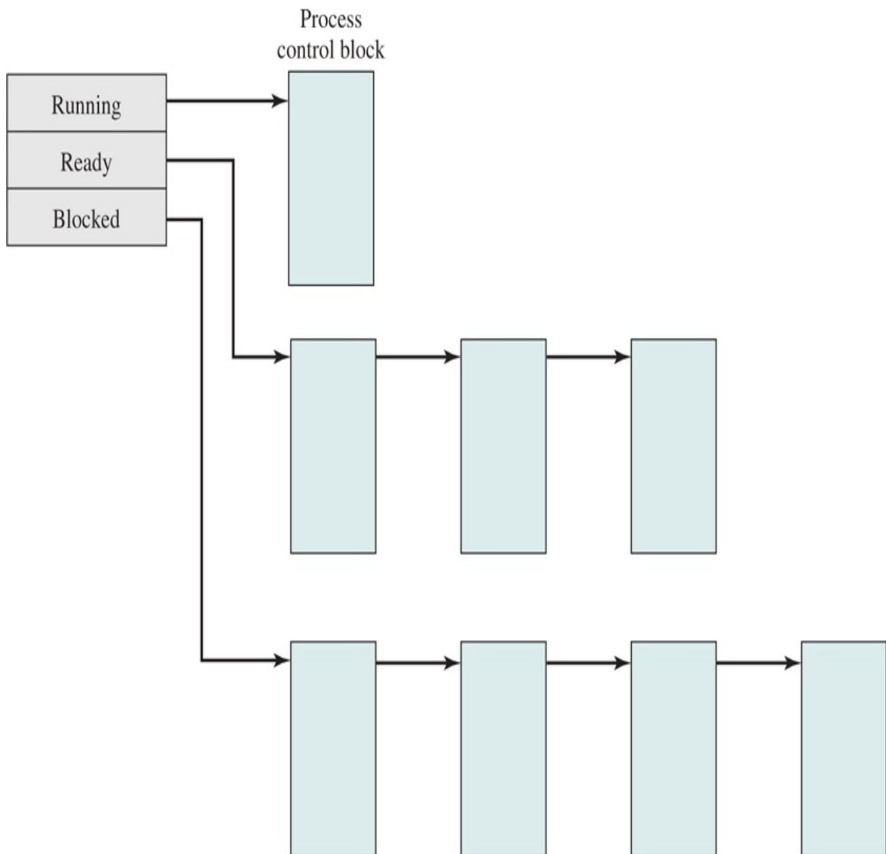
Figure 3.14 Process List Structures
