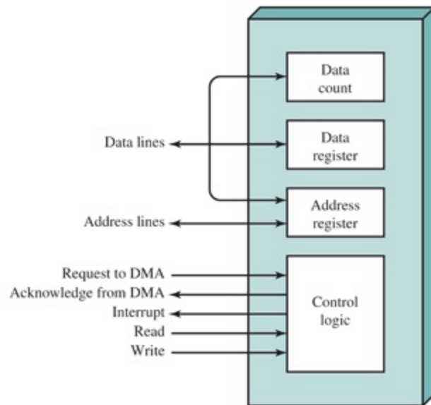
Figure 11.2 Typical DMA Block Diagram
