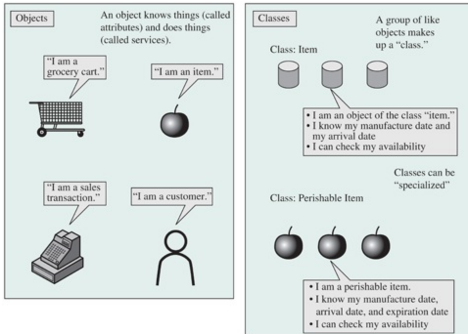
Figure D.2 Object Concepts
