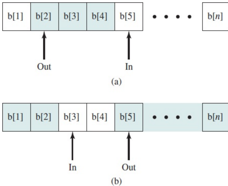
Figure 5.15 Finite Circular Buffer for the Producer/Consumer Problem
