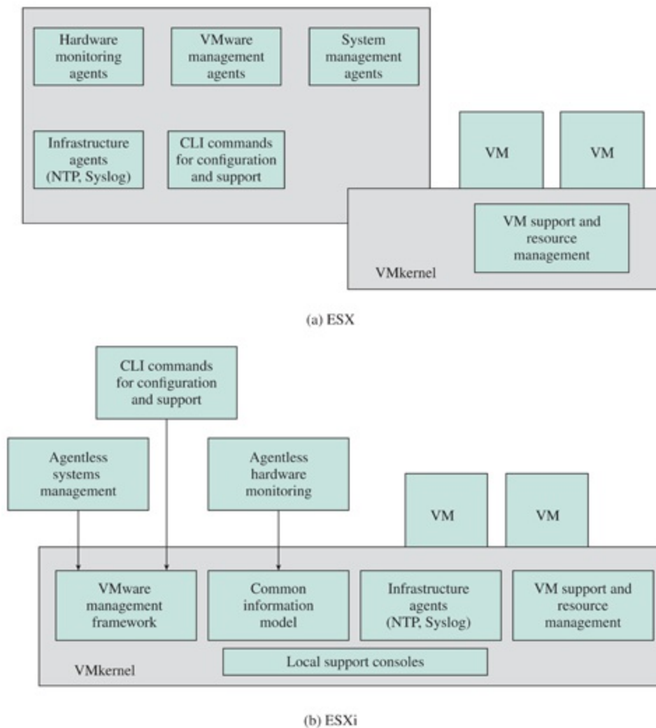
Figure 14.9 ESX and ESXi
