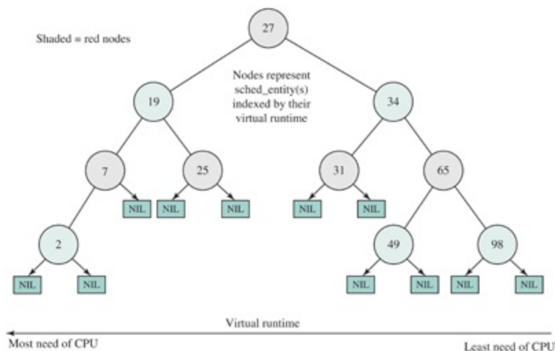
Figure 10.11 Example of Red Black Tree for CFS
