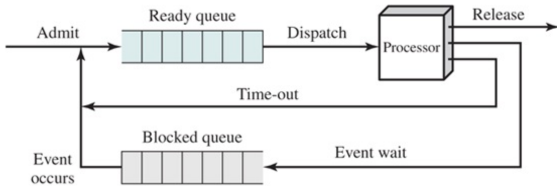
(a) Single blocked queue
