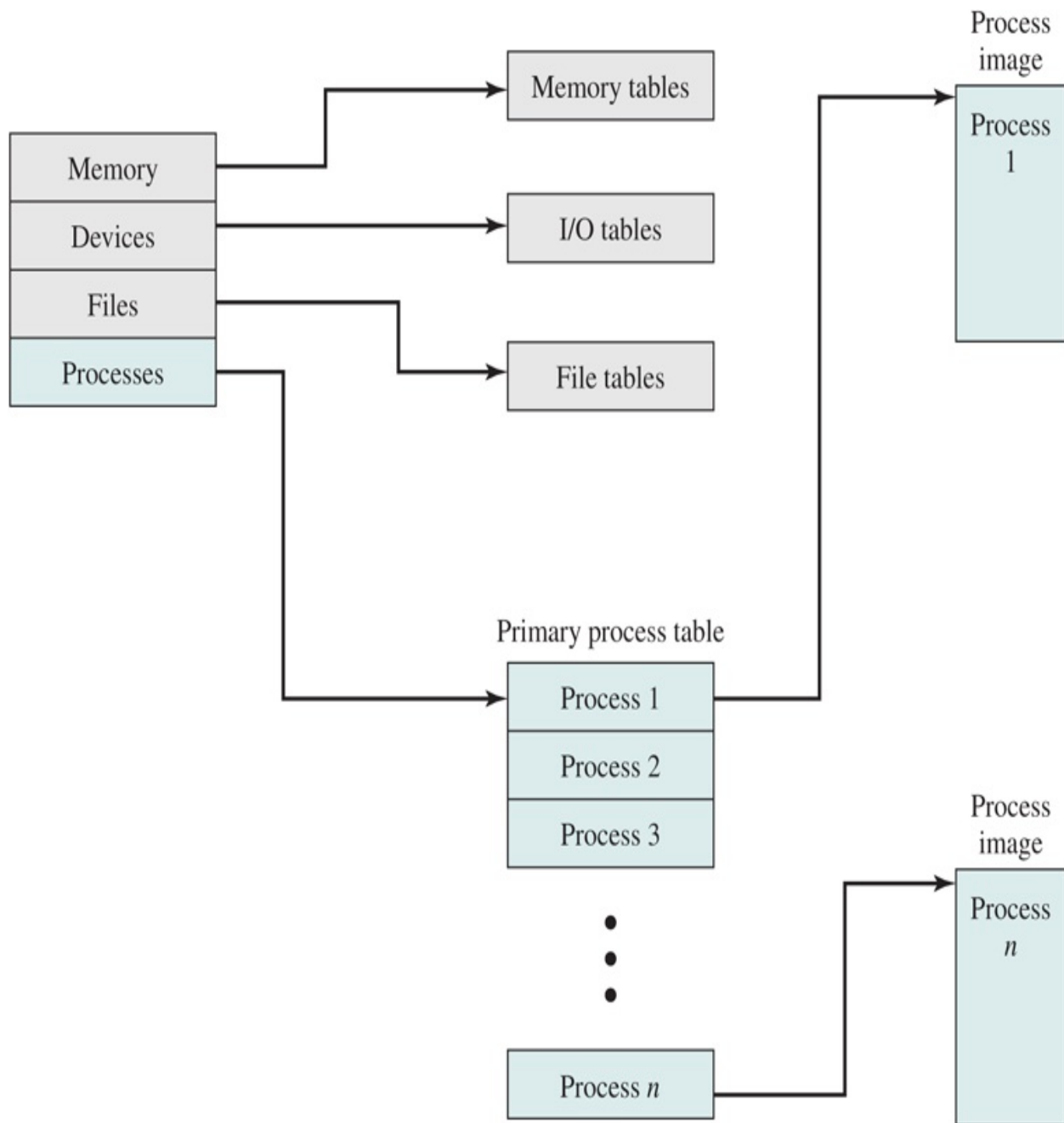
Figure 3.11 General Structure of Operating System Control Tables
