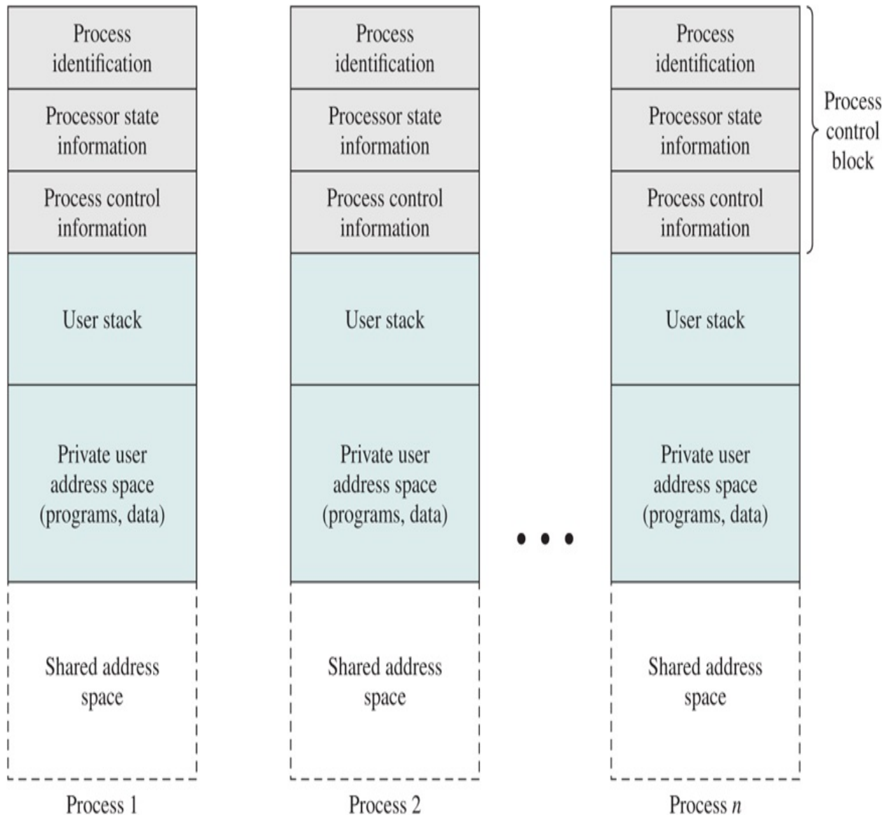
Figure 3.13 User Processes in Virtual Memory
