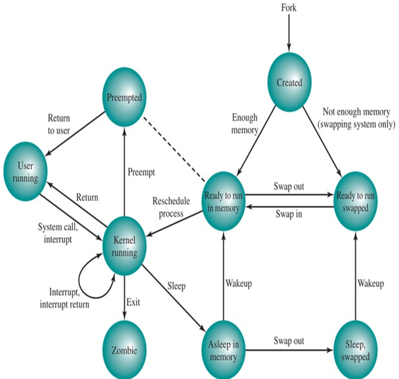
Figure 3.17 UNIX Process State Transition Diagram
