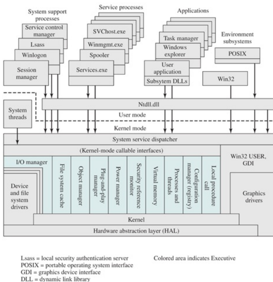
Figure 2.14 Windows Internals Architecture [ RUSS11 ]
