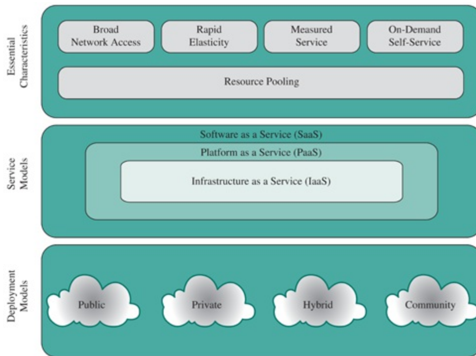
Figure 16.1 Cloud Computing Elements
