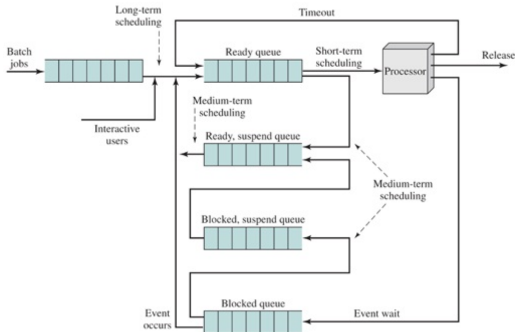
Figure 9.3 Queueing Diagram for Scheduling
