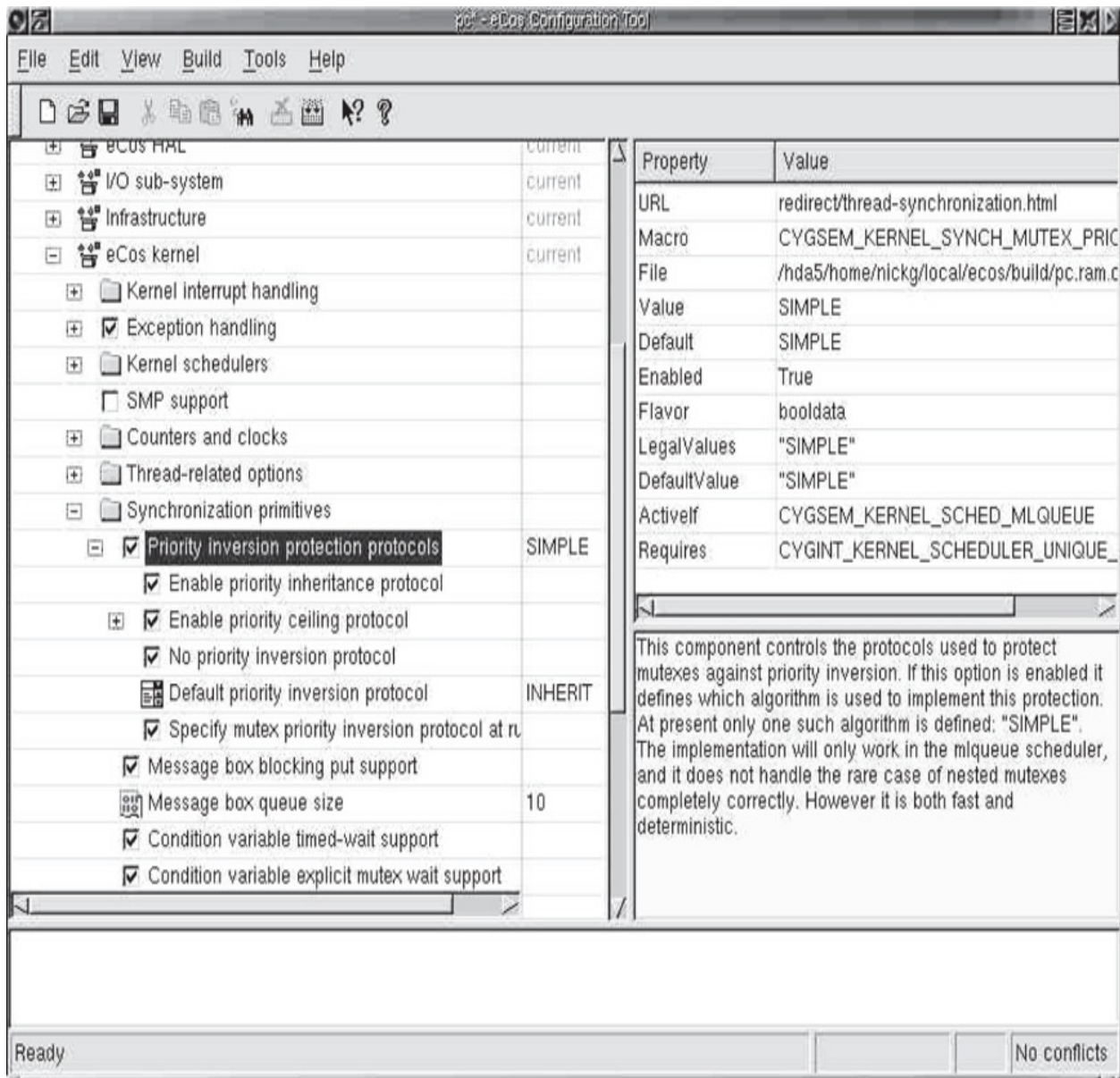
Figure Q.2 eCos Configuration Tool - Kernel Details
