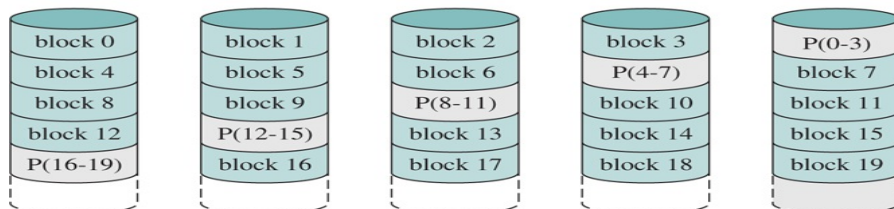
(f) RAID 5 (block-interleaved distributed parity)
