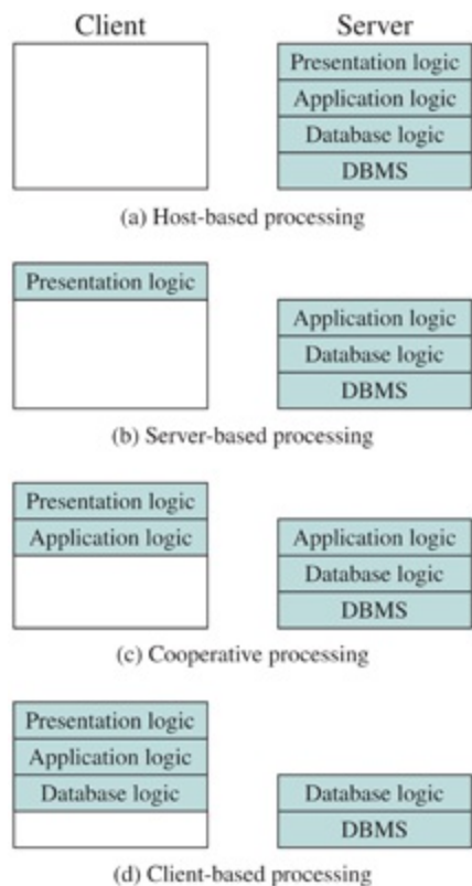
Figure 18.5 Classes of Client/Server Applications
