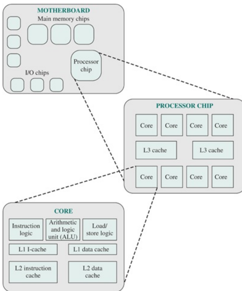
Figure 13.2 Simplified View of Major Elements of a Multicore
