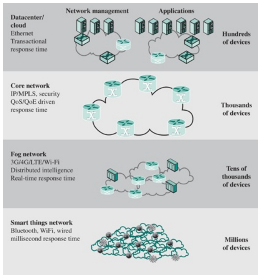
Figure 16.12 The IoT/Cloud Context
