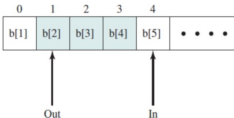
Figure 5.11 Infinite Buffer for the Producer/Consumer Problem
