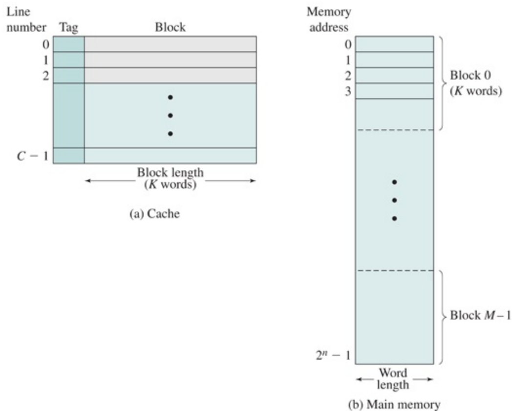
Figure 1.17 Cache/Main Memory Structure
