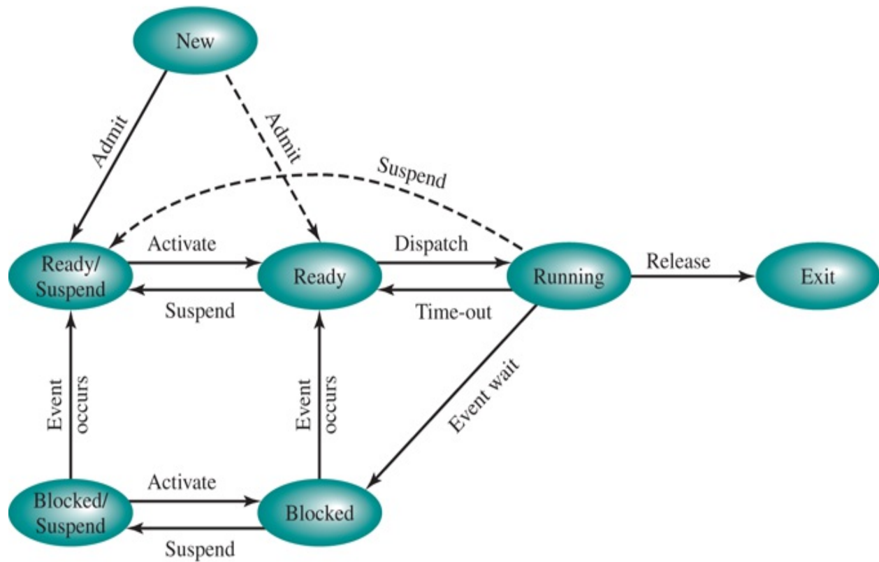
(b) With two Suspend states
