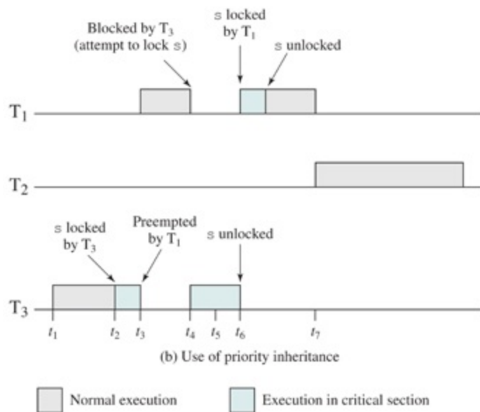
Figure 10.9 Priority Inversion
