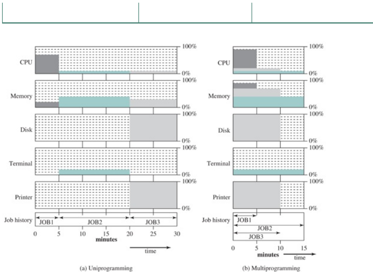
Figure 2.6 Utilization Histograms
