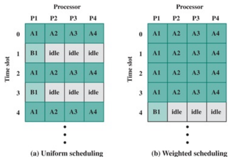
Figure 10.2 Gang Scheduling
