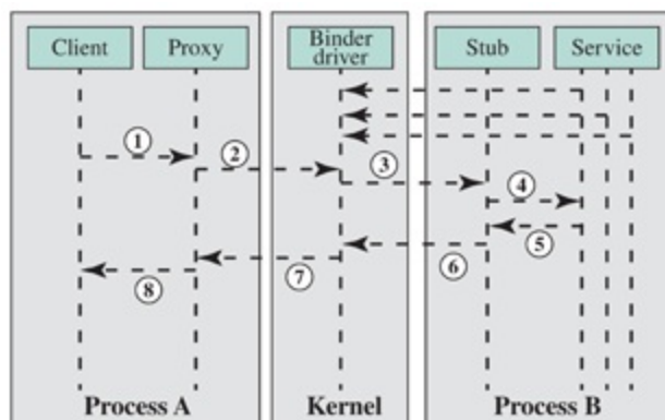
Figure 6.16 Binder Operation
