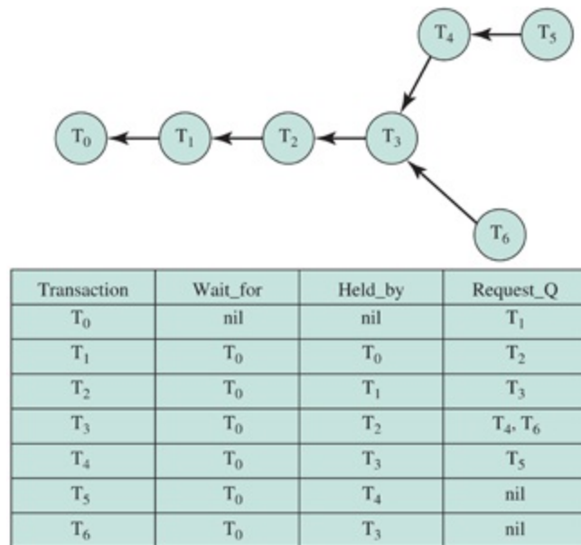
(a) State of system before request
