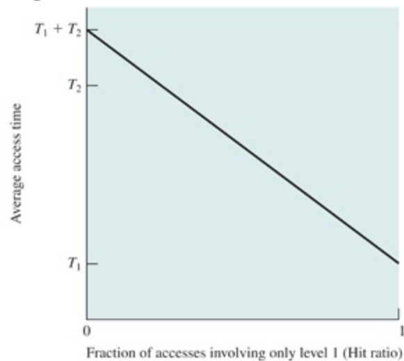
Figure 1.15 Performance of a Simple Two-Level Memory
