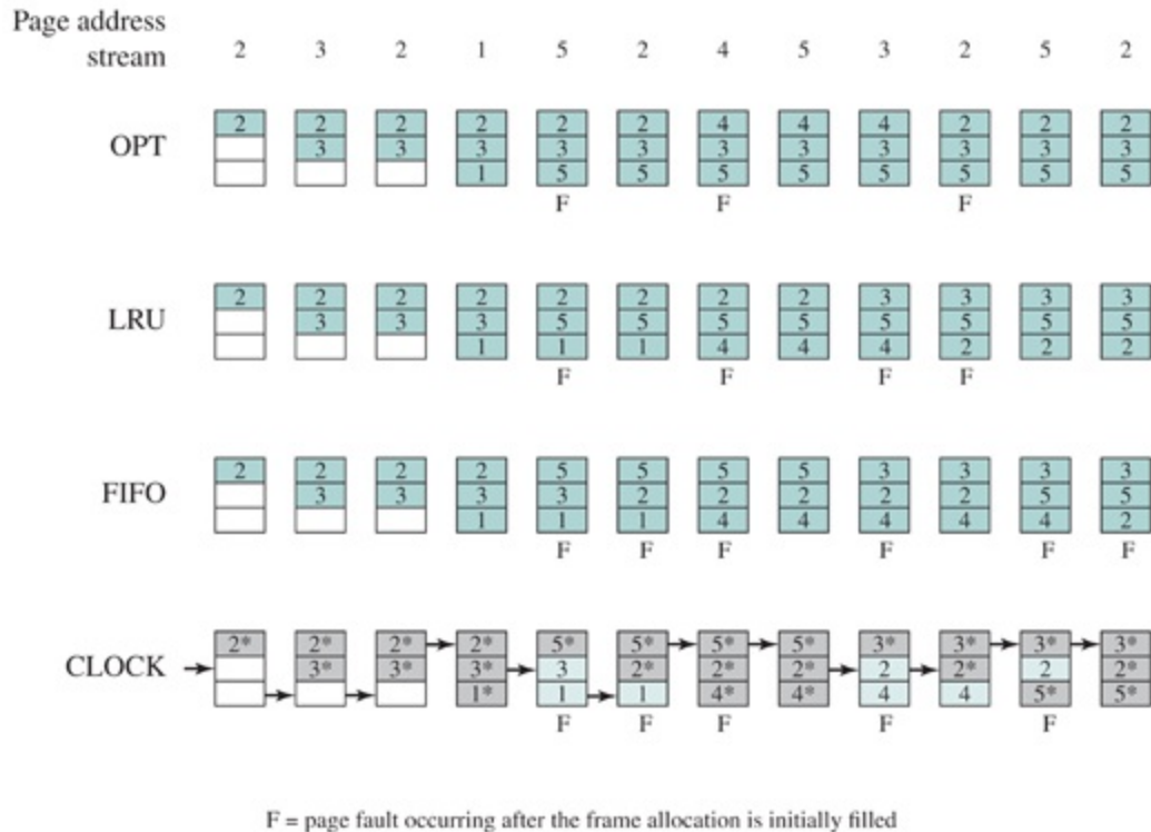
Figure 8.14 Behavior of Four Page Replacement Algorithms
