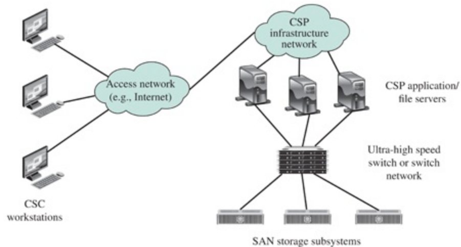
(b) Configuration with storage area network (SAN)
