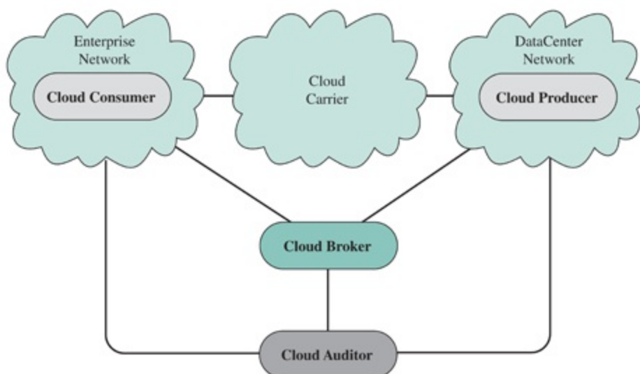
Figure 16.4 Interactions Between Actors in Cloud Computing
