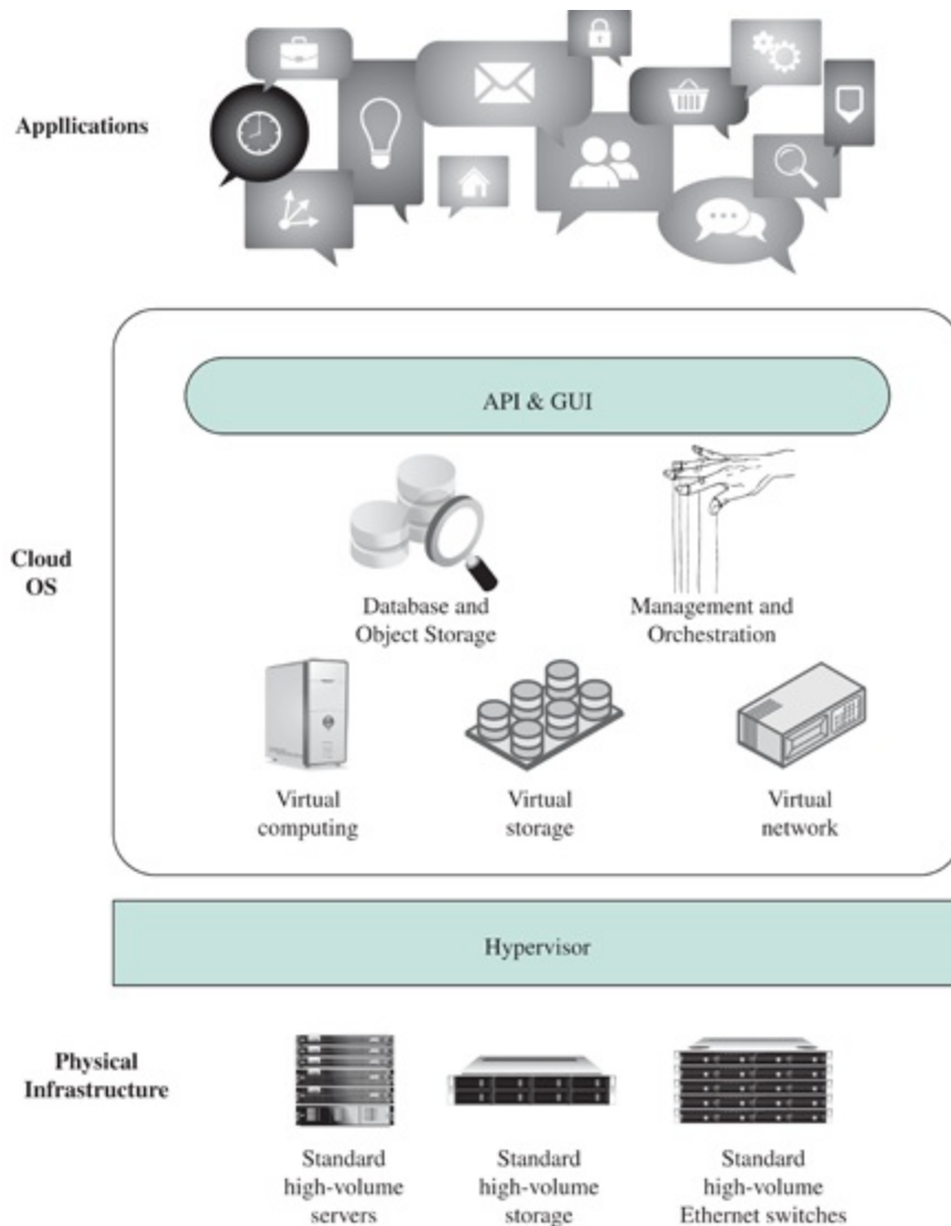
Figure 16.6 Cloud Operating System Concept
