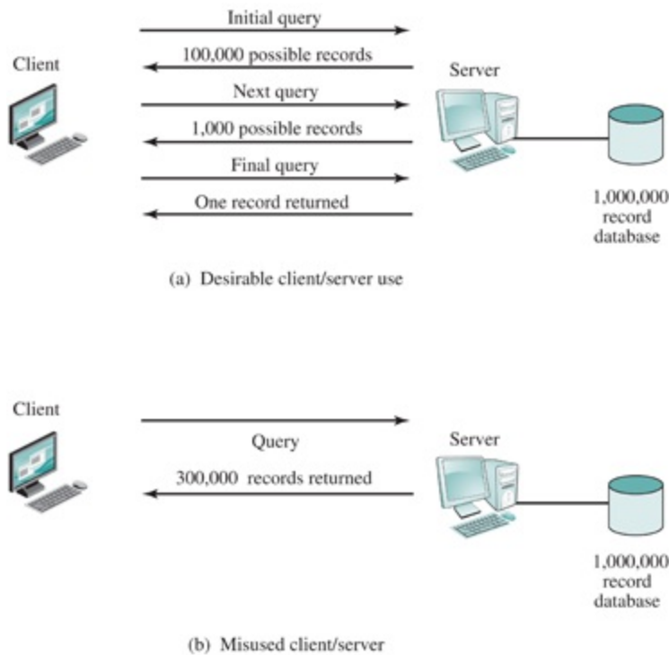
Figure 18.4 Client/Server Database Usage
