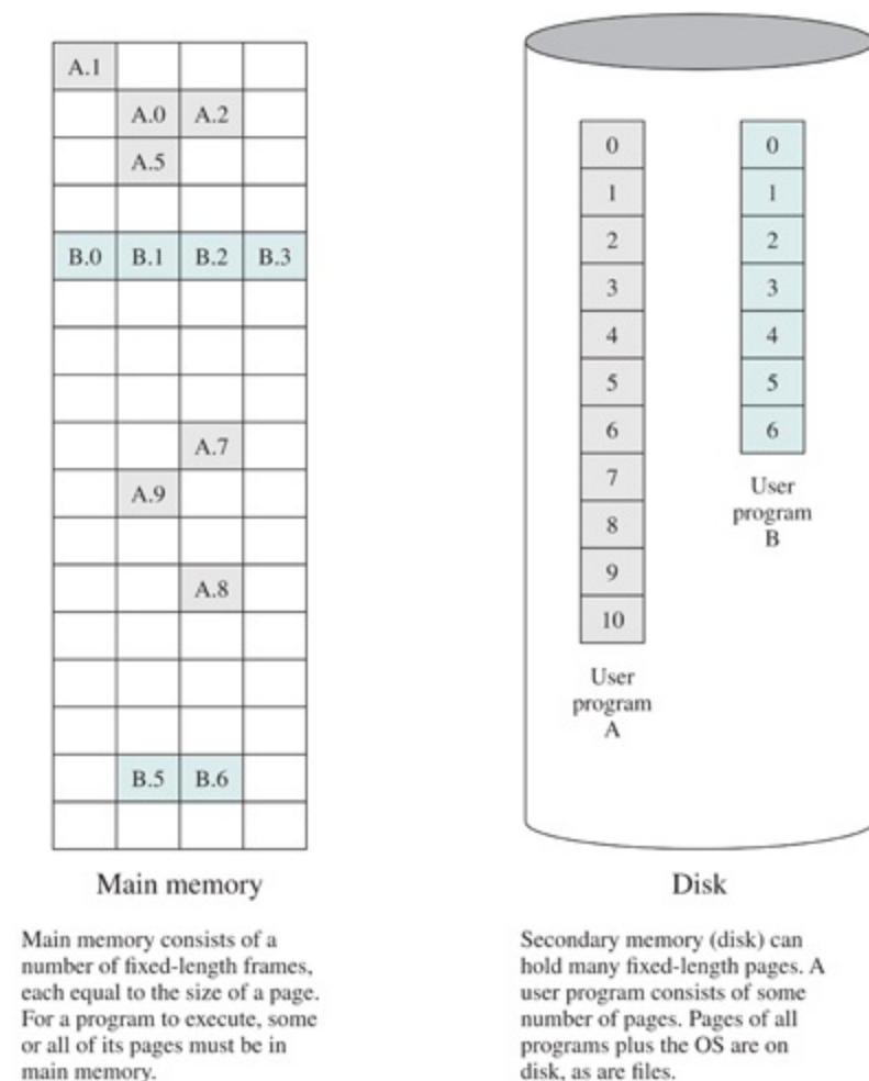
Figure 2.9 Virtual Memory Concepts
