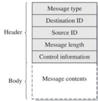
Figure 5.22 General Message Format
