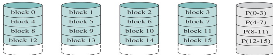
(e) RAID 4 (block-interleaved parity)
