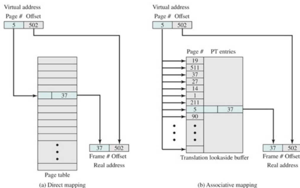
Figure 8.8 Direct versus Associative Lookup for Page Table Entries
