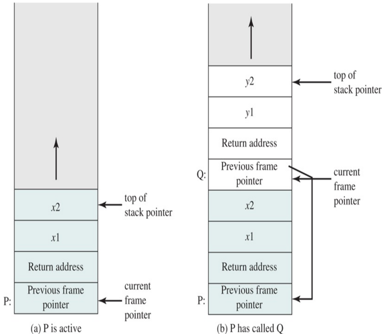
Figure P.4 Stack Frame Growth Using Sample Procedures P and Q
