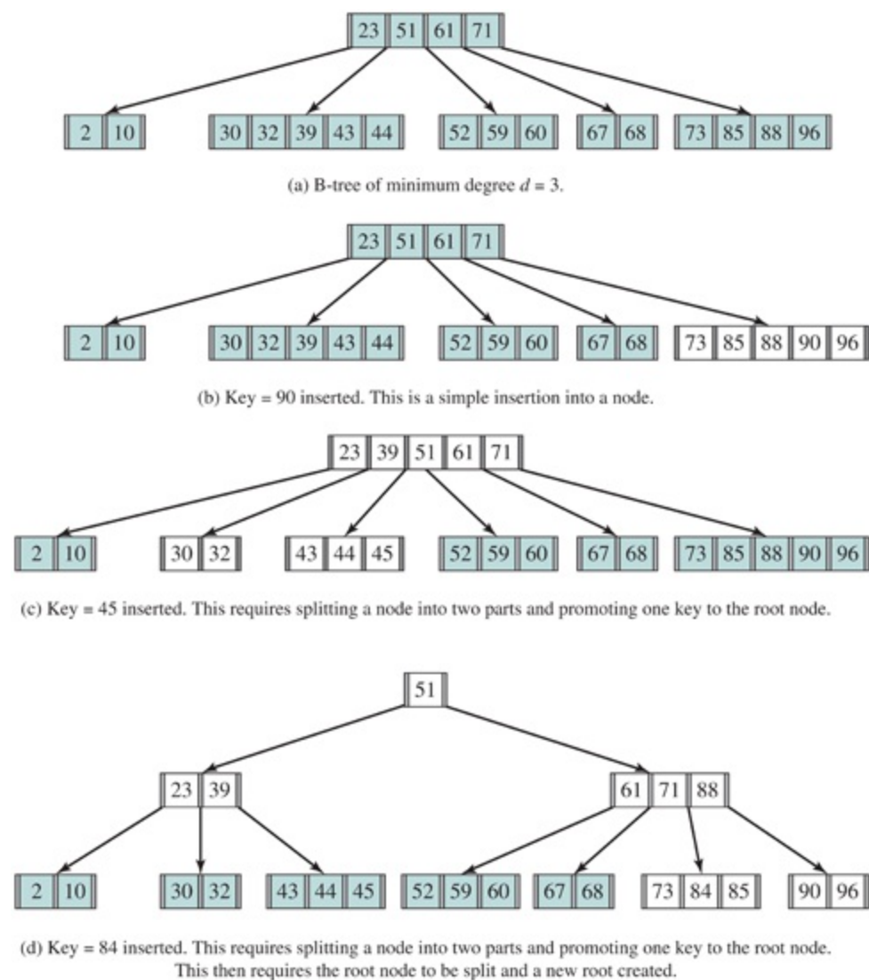
Figure 12.5 Inserting Nodes into a B-tree
