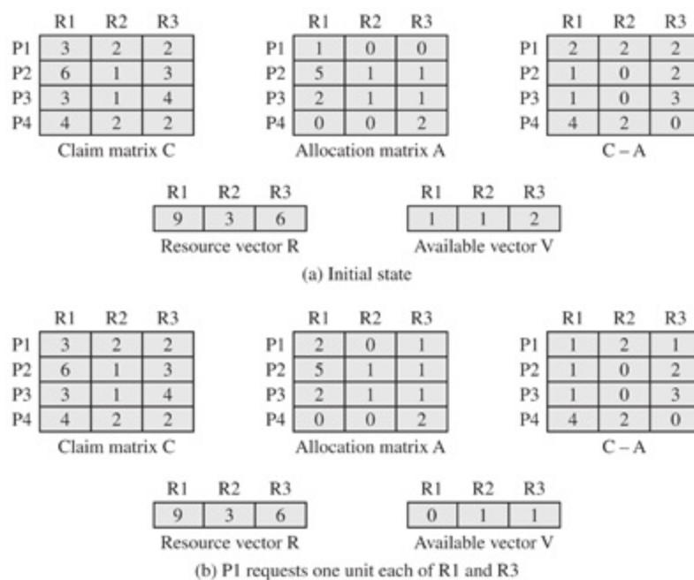
Figure 6.8 Determination of an Unsafe State
