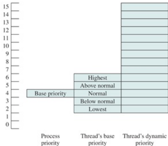
Figure 10.15 Example of Windows Priority Relationship
