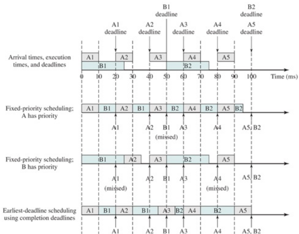
Figure 10.5 Scheduling of Periodic Real-Time Tasks with
