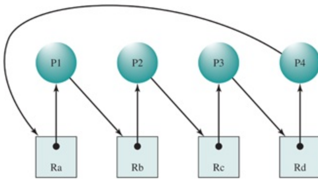
Figure 6.6 Resource Allocation Graph for Figure 6.1b
