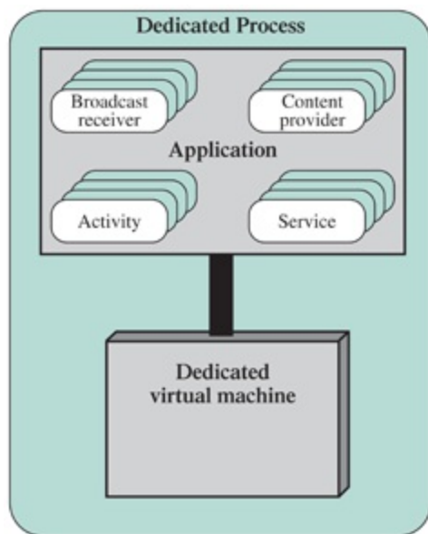
Figure 4.16 Android Application
