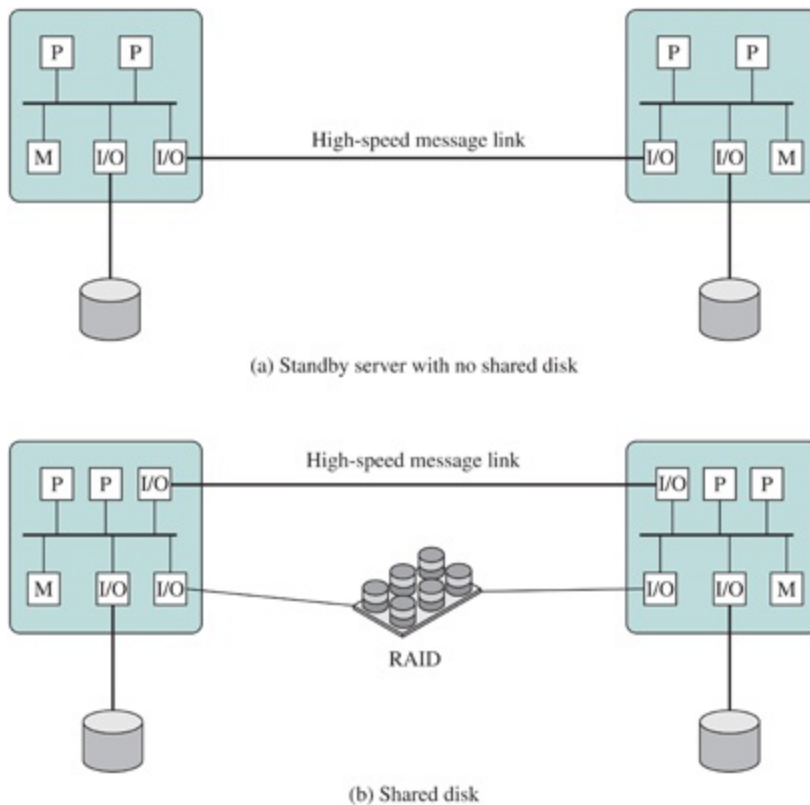
Figure 18.13 Cluster Configurations
