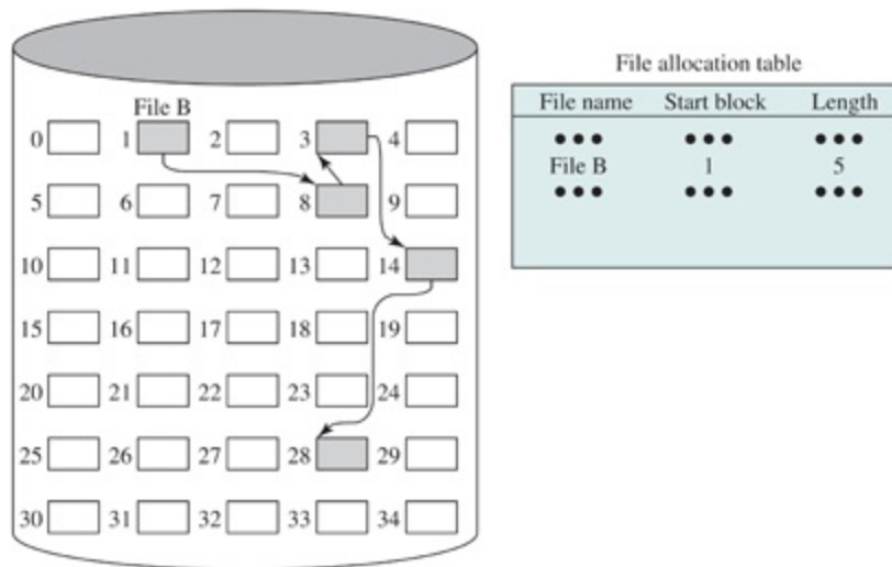
Figure 12.11 Chained Allocation
