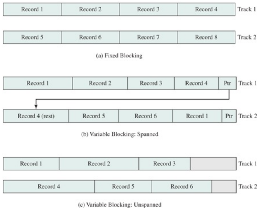
Figure 12.8 Record-Blocking Methods
