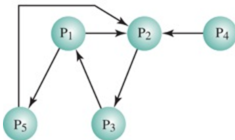
(b) Deadlock
