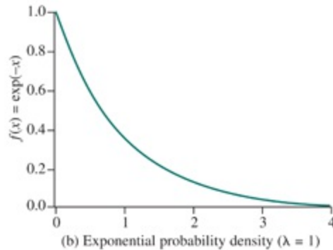
Figure 20.3 Some Probability Functions
