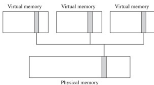
Figure 14.7 Page Sharing
