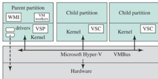
Figure 14.11 Hyper-V
