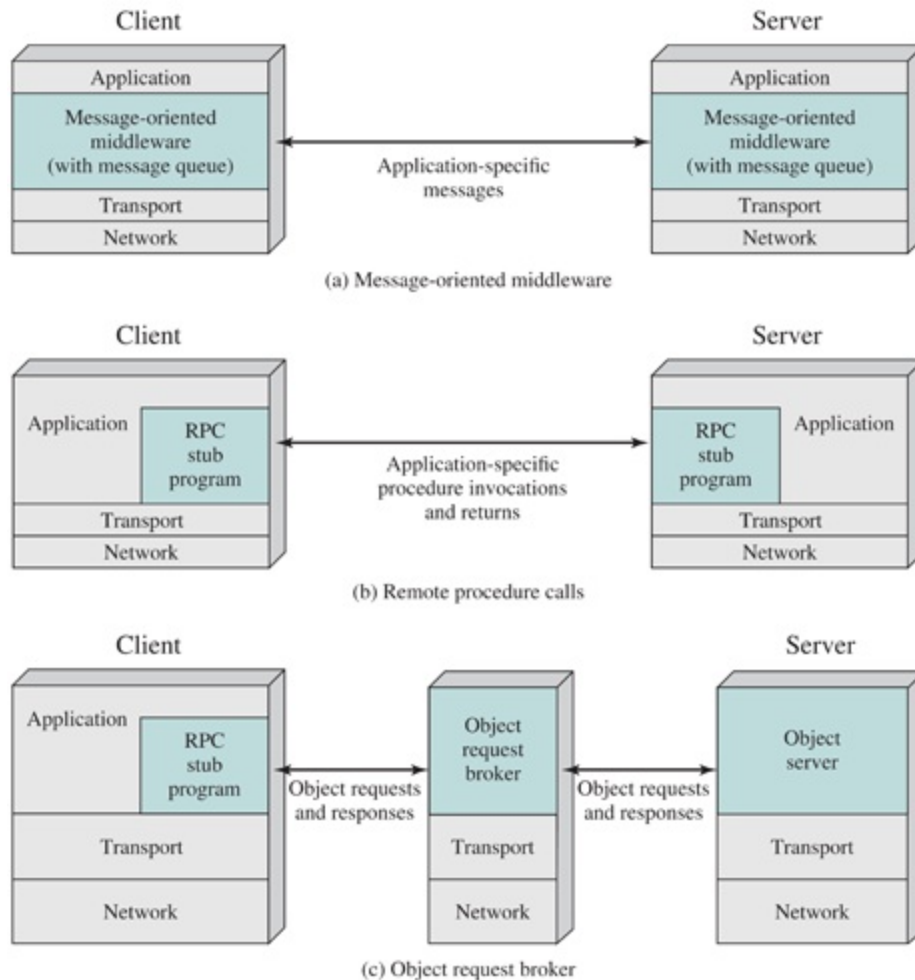
Figure 18.10 Middleware Mechanisms
