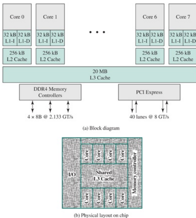
Figure 1.20 Intel Core i7-5960X Block Diagram
