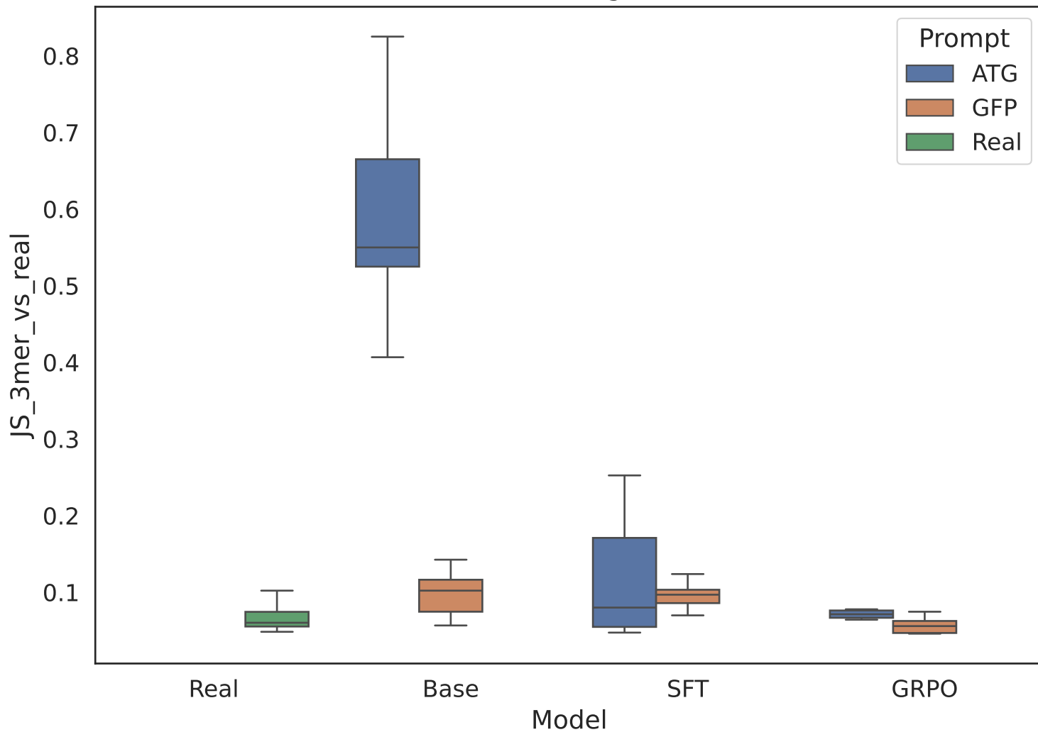
3-mer Divergence
