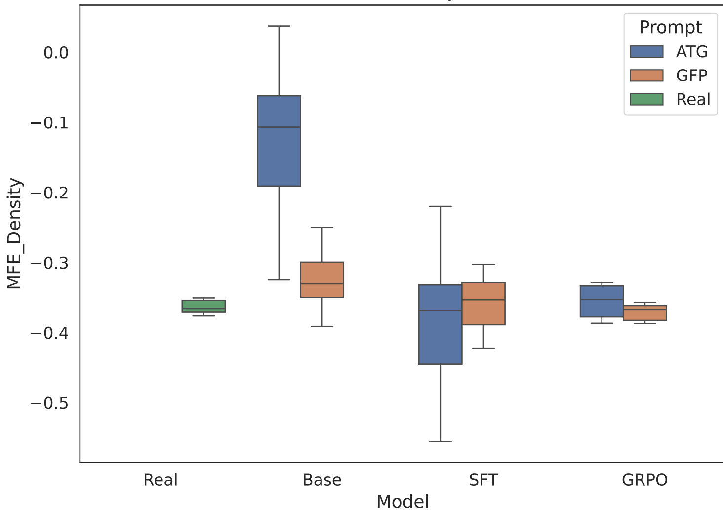
MFE Density
