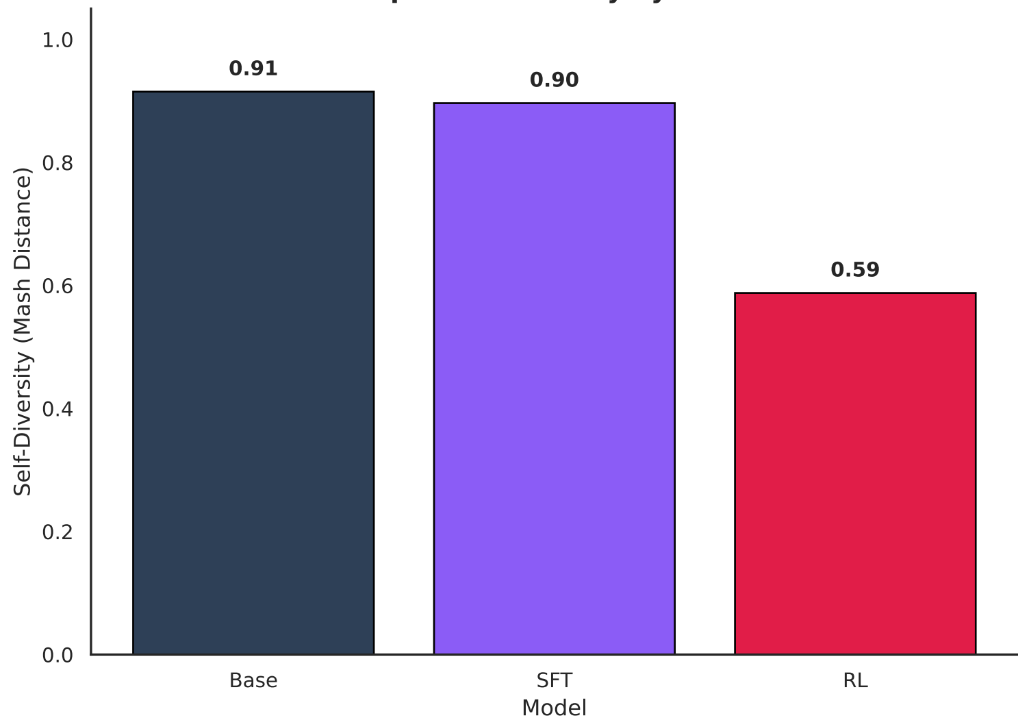
Sequence Diversity by Model
