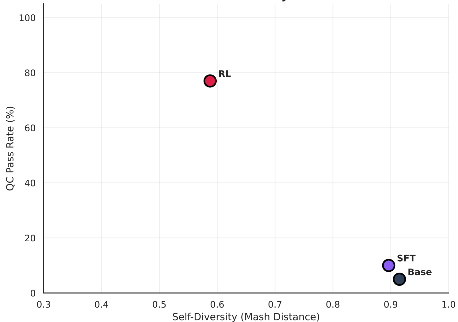
Pass Rate vs. Diversity Trade-off
