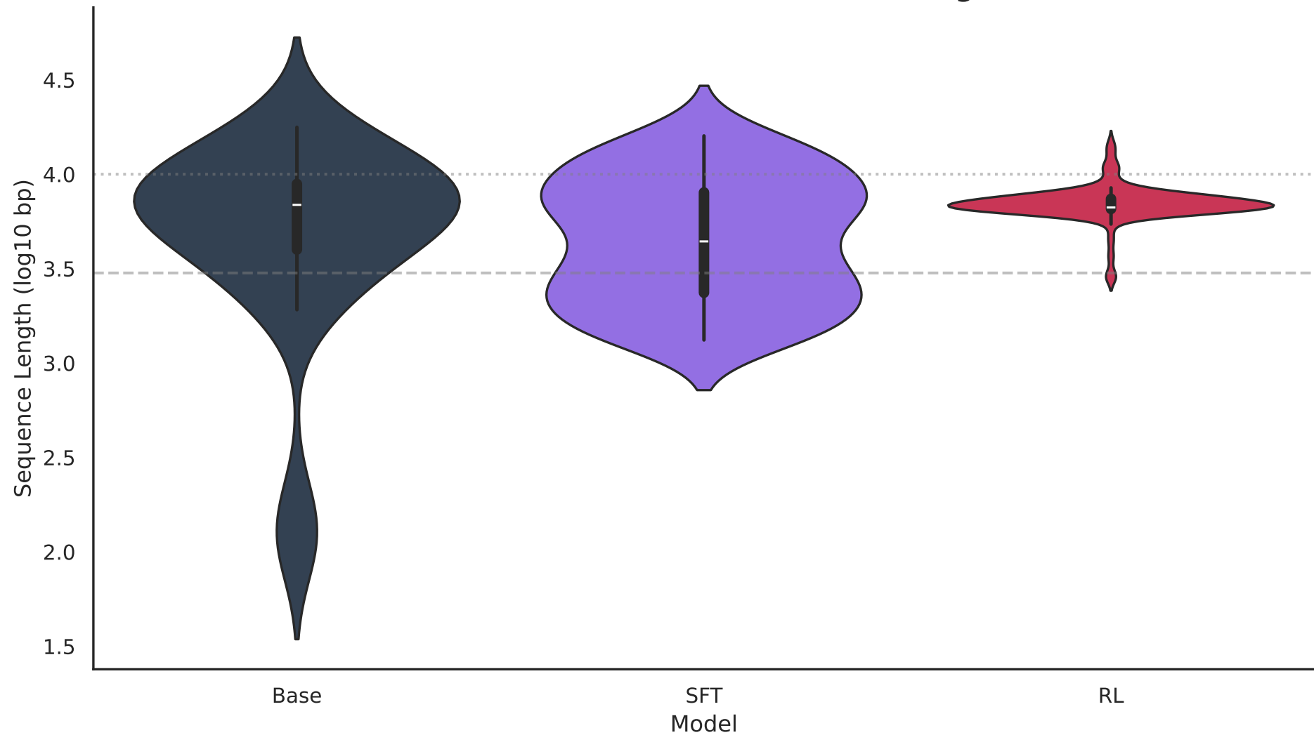
Distribution of Generated Plasmid Lengths
