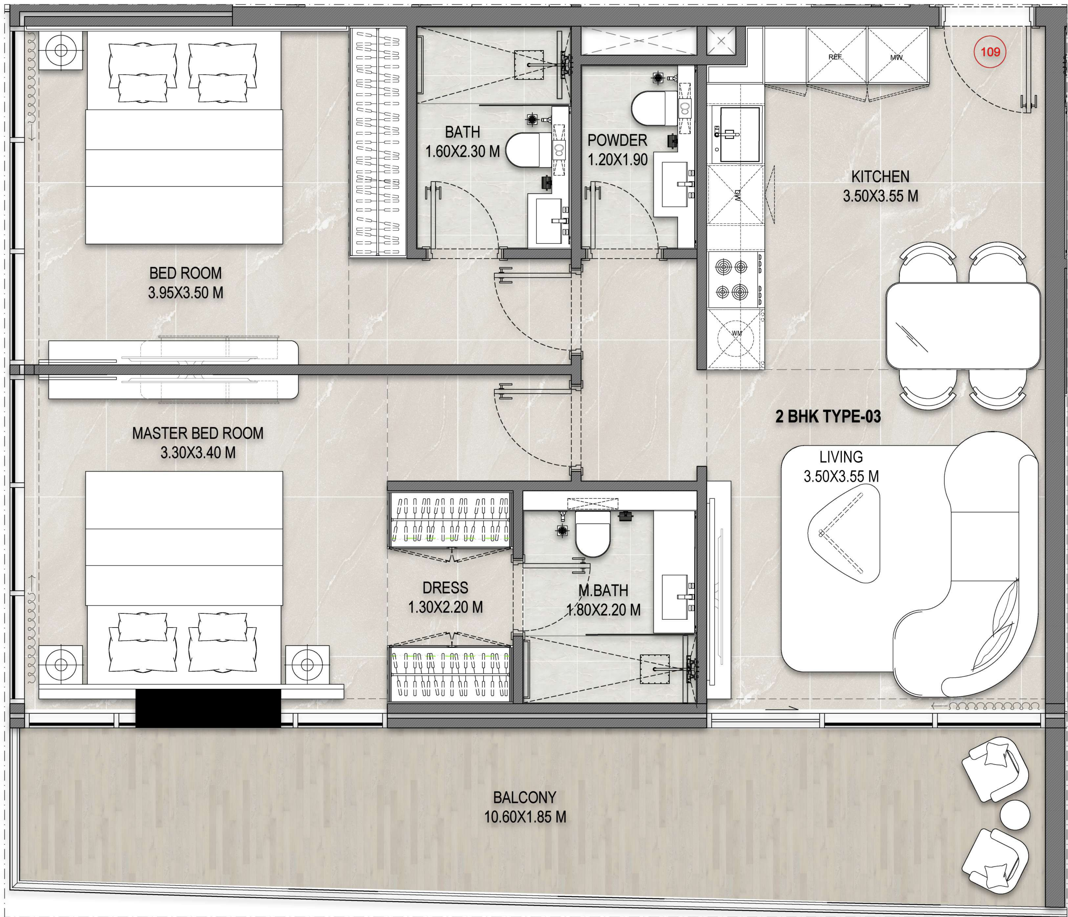
01 2BHK TYPE-03 SCALE 1:100@A1
