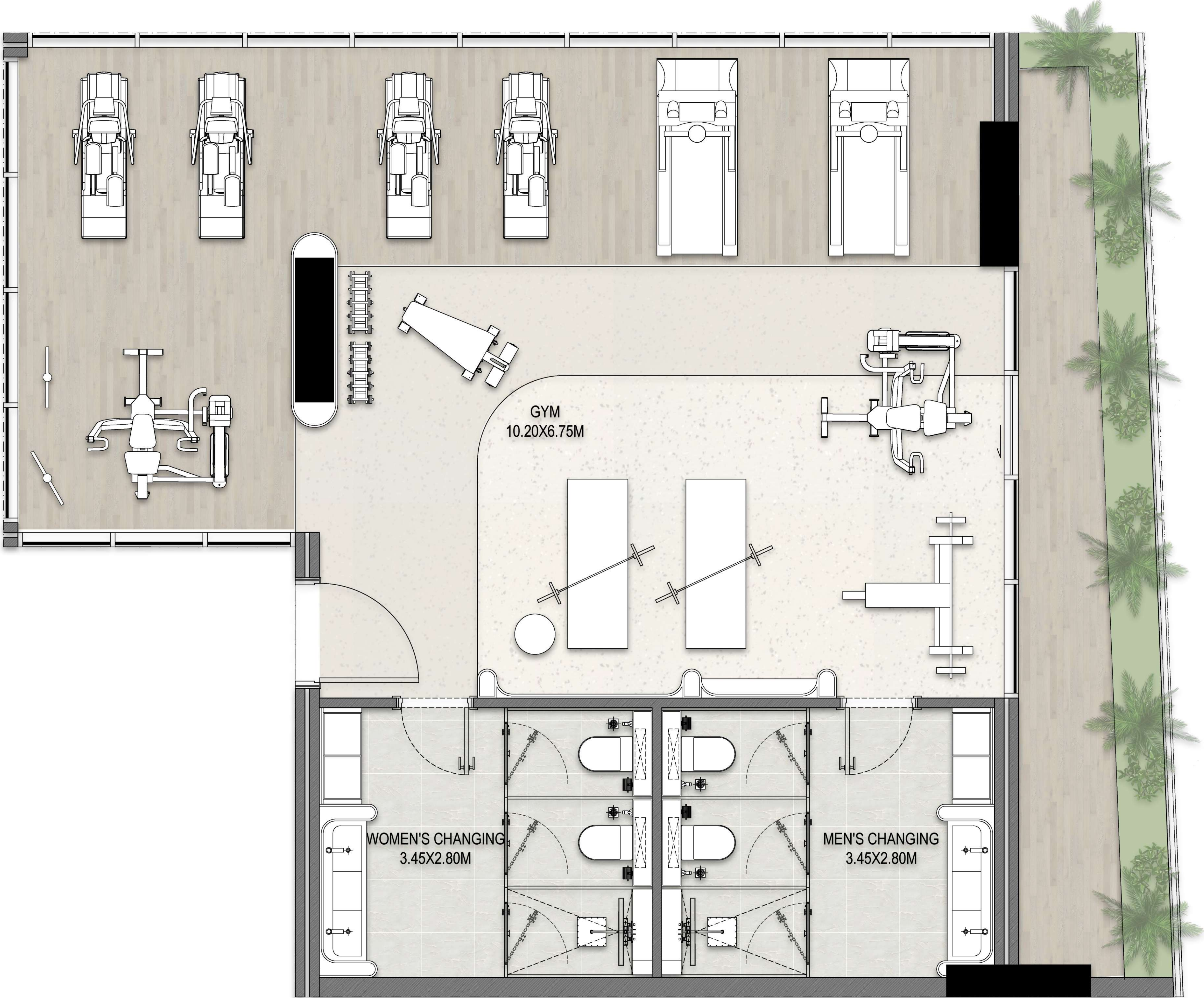
01 GYM & LOCKERS SCALE 1:100@A1
