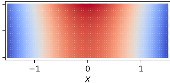
analytical w ( \Lambda^* = 0.964 , MAC = 1.000)
