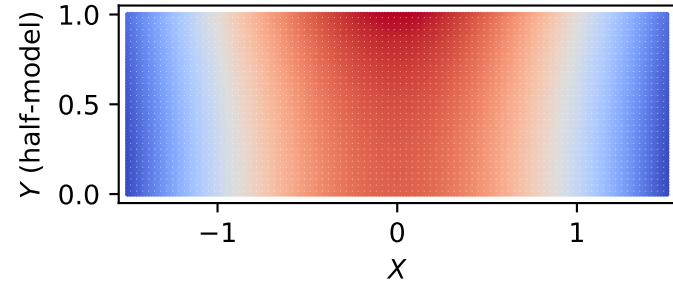
FE U_Z (mode 4, \Lambda = 0.96347 )
