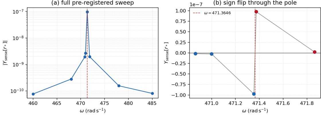
Figure 3: Segmented-electrode sensing admittance Y_{\text{sense}}[r_*] near the free-free short-circuit fundamental ( 471.3646 \text{ rad s}^{-1} ), r_F = 0.35 \text{ m} , r_* = 0.30 \text{ m} . (a) magnitude across the pre-registered validation sweep; (b) sign flip through the pole, undamped. Not a dense resonance curve – the nine points are the pre-registered validation gate, not a fitted or interpolated response.
