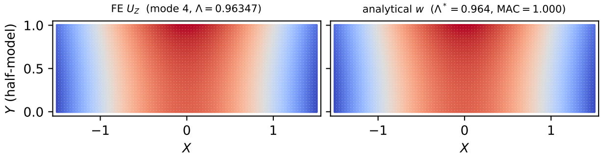
Figure 2: Half-model first symmetric flexural mode at \ell/b = 1.5 . Left: SHELL281 U_Z (mode 4, \Lambda_{FE} = 0.96347 ). Right: analytical w at \Lambda^* = 0.964 , \text{MAC} = 1.000 .
