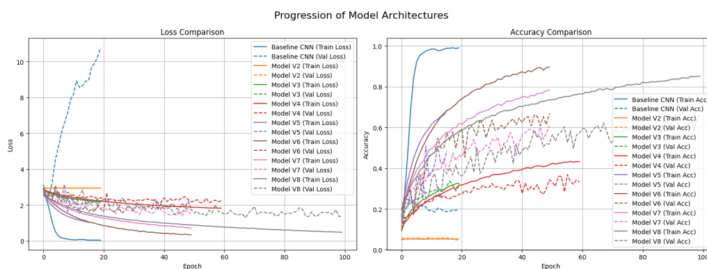
Figure 2: Performance Comparison of CNN Architectures from Scratch
