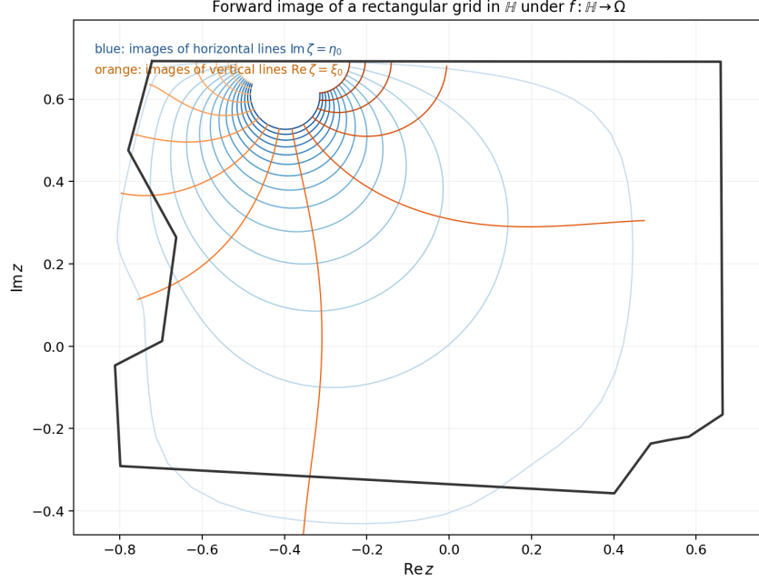
Figure 8: Forward image of a rectangular grid in \mathbb{H} under the SC map f . Blue curves are images of horizontal lines \text{Im } \zeta = \eta_0 for \eta_0 \in [0.03, 1.8] ; orange curves are images of vertical lines \text{Re } \zeta = \xi_0 for \xi_0 \in [-2.4, 2.4] . The two families remain orthogonal throughout \Omega , confirming conformality of f . Compare with Figure 7(b), which shows the same type of conformal grid labelled as flow streamlines and equipotentials.
