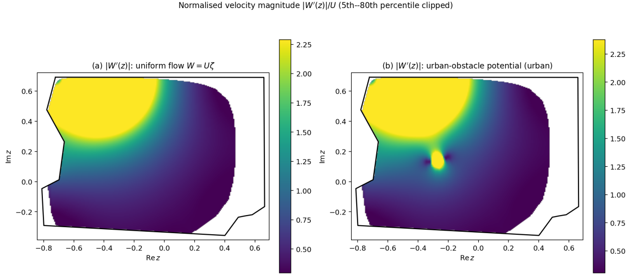
Figure 10: Normalised velocity magnitude |W'(z)|/U for the two flow models. (a) Uniform flow: speed rises sharply near polygon vertices where f'(\zeta_k) \rightarrow 0 . (b) Urban-obstacle potential: two additional bright regions on the flanks of the downtown core quantify the “local acceleration” visible in Figure 9. Colour bar clipped to the 5th–80th percentile to suppress the finite-grid blow-up at vertex branch points while keeping the flank acceleration visible.
