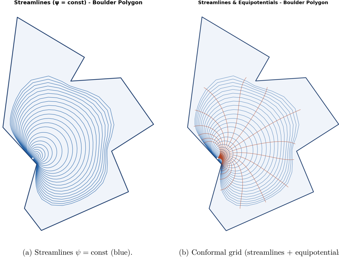
Figure 2: Uniform flow W = U\zeta in the 11-vertex Boulder polygon \Omega . Streamlines are the forward images of horizontal lines \text{Im}\zeta = \eta_0 in \mathbb{H} ; equipotentials are images of \text{Re}\zeta = \xi_0 . The SC map f : \mathbb{H} \rightarrow \Omega preserves angles locally, so the two families meet orthogonally throughout the interior. Grid resolution 400 \times 400 in \mathbb{H} ; 50 contours per family. Closed-streamline appearance is a topological consequence discussed above.
