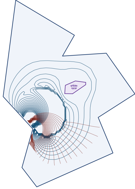
(b) Urban obstacle, potential (16).
