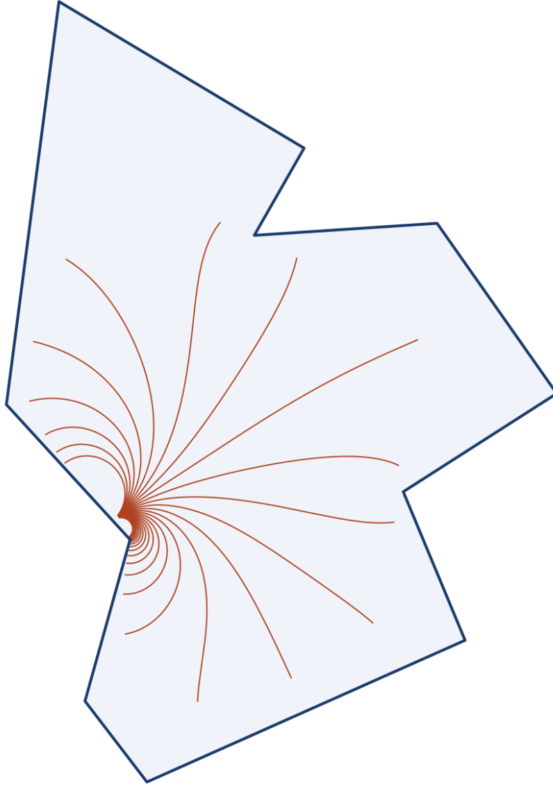
Figure 5: Equipotentials \phi = \text{const} for uniform flow W = U\zeta , shown alone. Each curve is the forward image of a vertical half-line \text{Re}\zeta = \xi_0 in \mathbb{H} . See Section 5.2.
