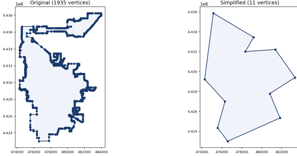
Figure 1: Boulder boundary before and after SC preprocessing. Left: original 1935-vertex TIGER/Line polygon [US Census Bureau, 2025]. Right: 11-vertex simplification after Douglas–Peucker reduction and iterative angle filtering with bounds \alpha_k \in [0.35\pi, 1.75\pi] . The simplified polygon is the domain \Omega for all subsequent SC computations.
