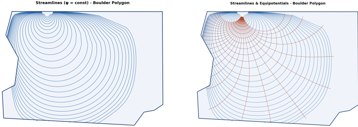
(a) Streamlines \psi = \text{const} (blue).
