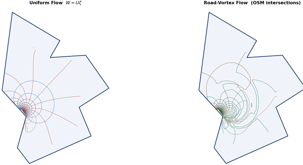
Figure 10: Side-by-side: uniform flow (left) vs. road-vortex flow (right). The road-vortex correction introduces organised local circulation absent from the uniform baseline, particularly along the Broadway and 28th St corridors.
