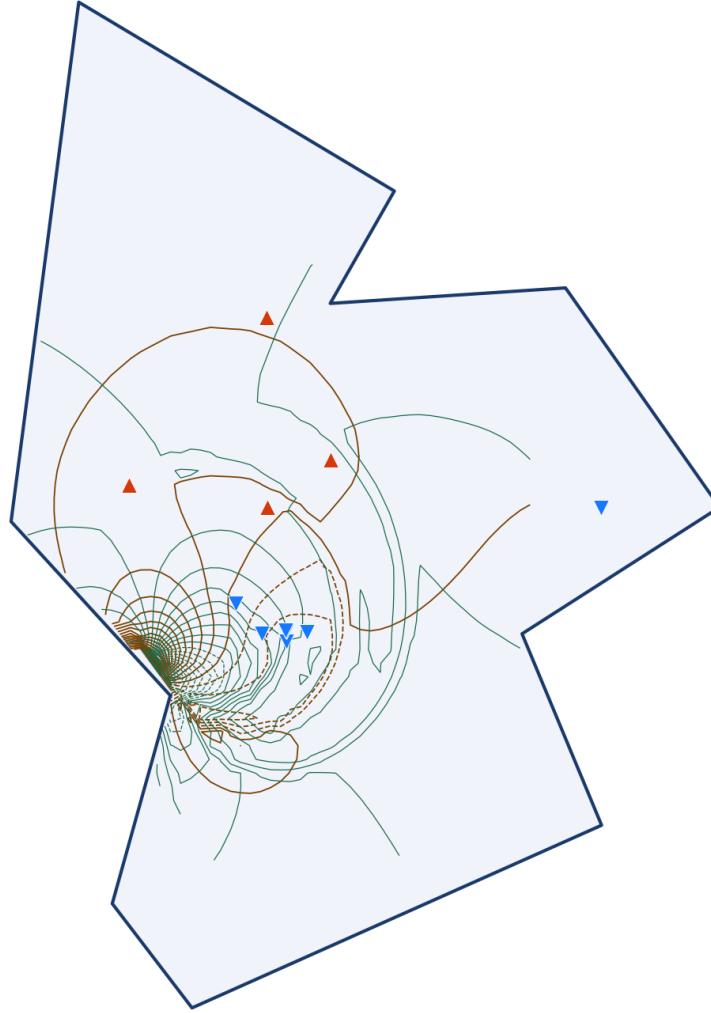
Figure 6: Road-vortex flow (44). Point vortices at 11 OSM road intersections (primary through tertiary roads). Orange triangles: CCW vortices north of the polygon centroid ( \Gamma > 0 ). Blue triangles: CW vortices south ( \Gamma < 0 ). Local eddies are visible around each intersection; the CCW/CW dipole pattern is consistent with Boulder's prevailing westerly flow shear.
