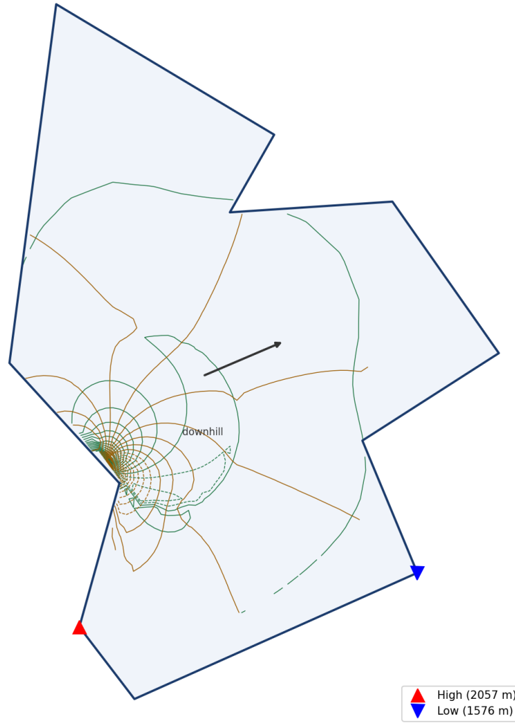
Figure 4: Terrain-corrected streamlines (green) and equipotentials (amber) under potential (43). Red triangles: high-elevation source vertices (2057 m); blue triangles: low-elevation sink vertices (1576 m). Streamlines deflect eastward relative to the uniform baseline, reproducing the slope-driven wind pattern characteristic of Boulder's foothill terrain.
