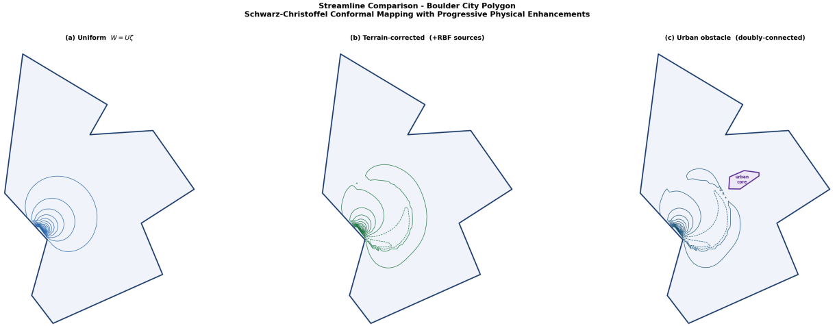
Figure 9: Three-way comparison: uniform, terrain-corrected, and urban-obstacle flow at identical contour levels. The progressive enrichment of the physical model is apparent in the streamline morphology of each panel.
