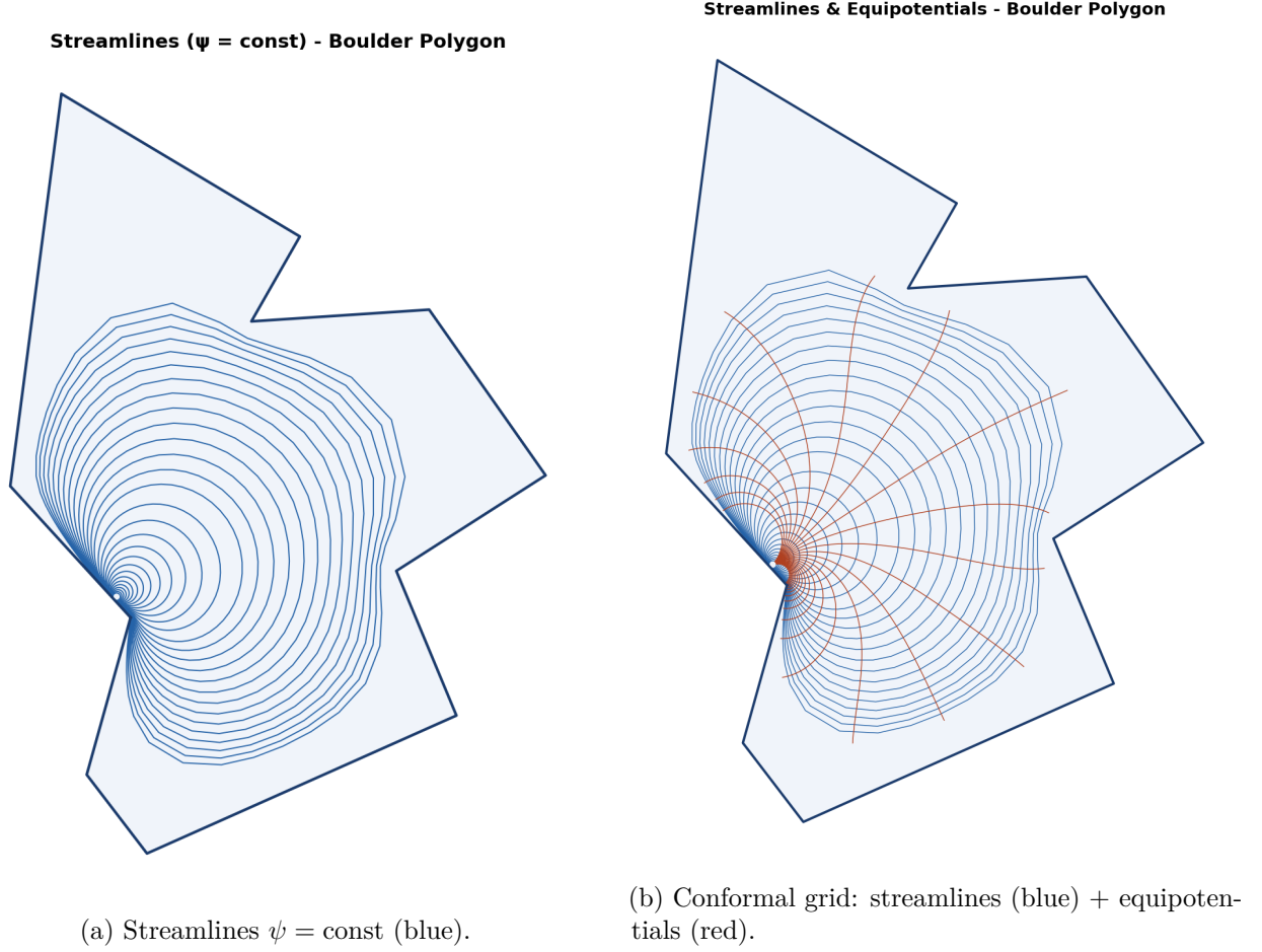
Figure 3: Uniform ideal flow W = U\zeta in \Omega . Streamlines are the forward images of horizontal lines \text{Im}(\zeta) = \eta_0 in \mathbb{H} ; equipotentials are images of vertical lines \text{Re}(\zeta) = \xi_0 . Orthogonality of the two families confirms conformality of the map.
