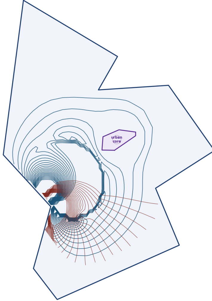
Figure 5: Doubly-connected flow potential (34). The downtown Boulder urban core (purple polygon) is treated as an impenetrable obstacle in \mathbb{H} . The Milne-Thomson circle theorem enforces \psi = \text{const} on the enclosing circle; the image term at \bar{\zeta}_0 preserves \psi = 0 on \partial\mathbb{H} . The achieved separation ratio \text{Im}(\zeta_0)/a \approx 5.36 yields an approximation error of \sim 3.5\% . See Figure 2(c) for the deflection pattern around the urban core.
