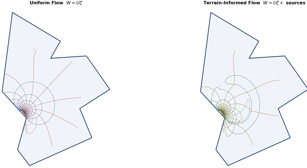
Figure 8: Side-by-side: uniform flow (left) vs. terrain-corrected flow (right) at the same contour levels. The eastward shift of streamlines under the terrain correction (43) is evident throughout the western portion of the domain.
