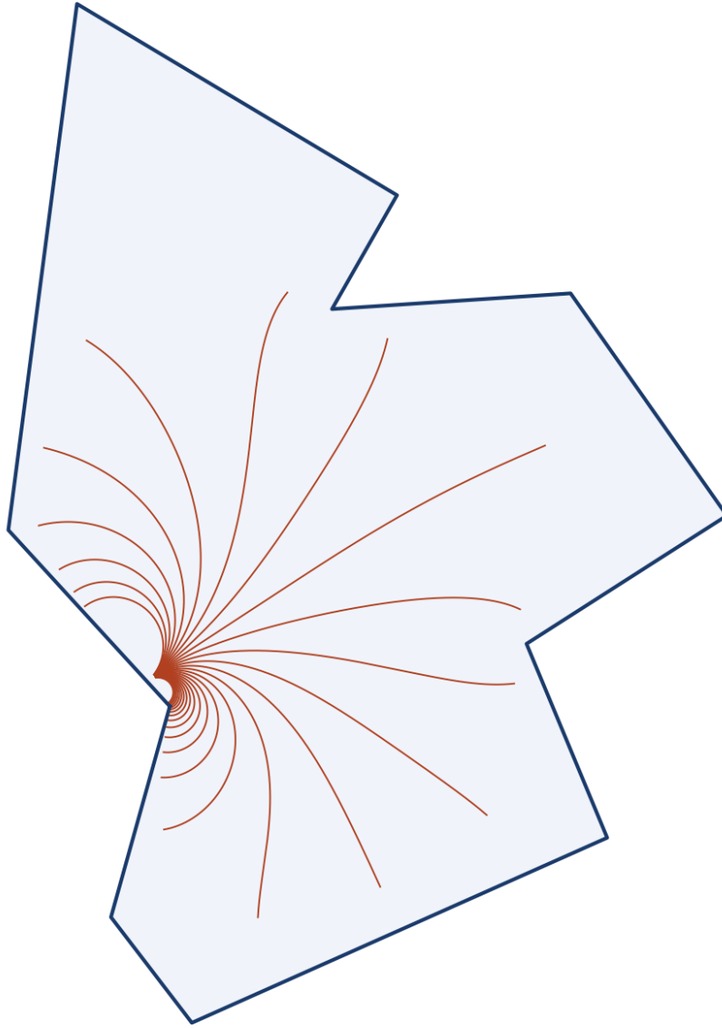
Figure 7: Equipotential lines ( \phi = \text{const} , red) for uniform flow W = U\zeta , shown without streamlines for clarity. Each curve is the forward image of a vertical half-line \text{Re}(\zeta) = \xi_0 in \mathbb{H} .
