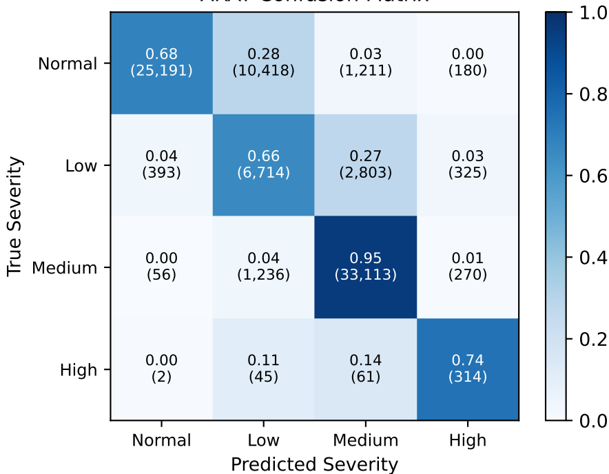
ARAT Confusion Matrix
