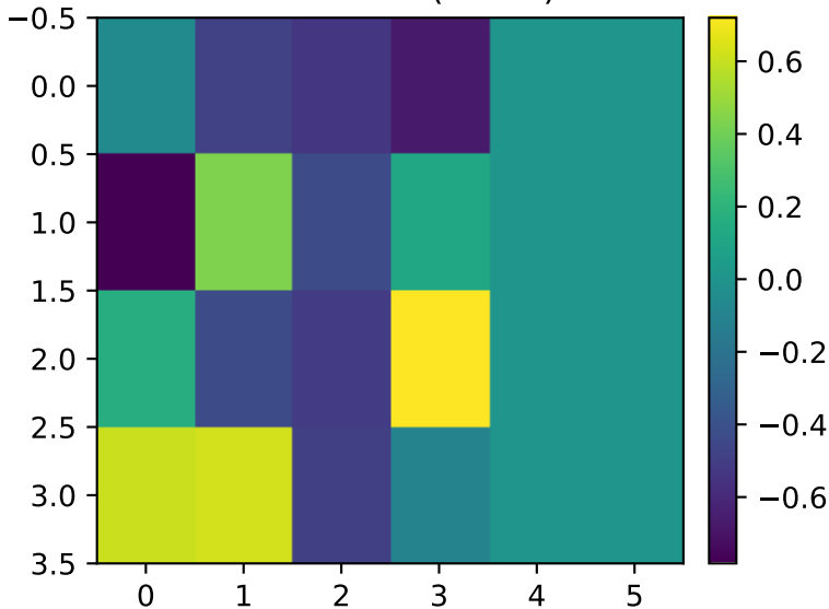
U from A^T A ( n \times m )
