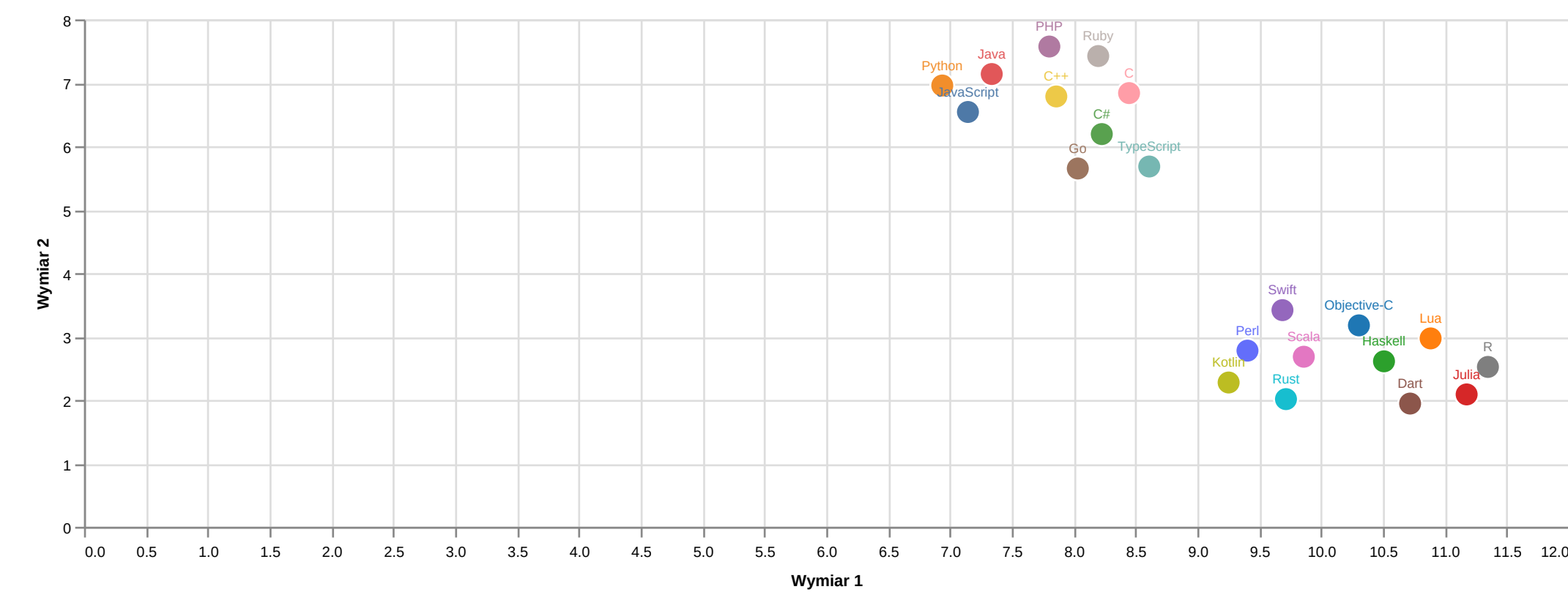
TriMAP
