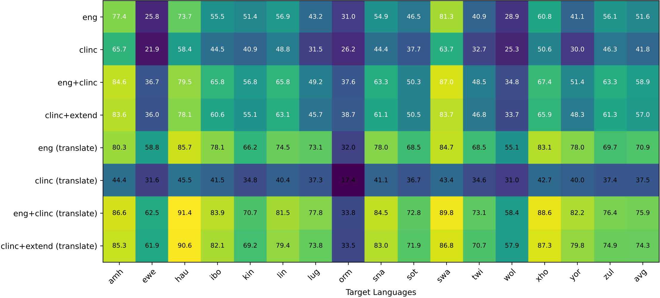
AfroXLMR-76L Intent Detection
