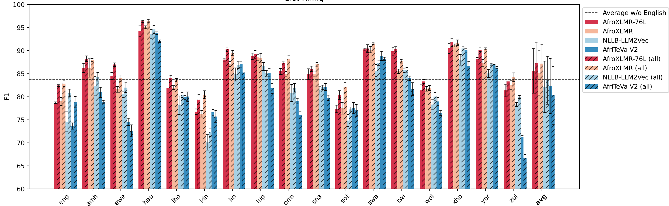
Slot Filling
