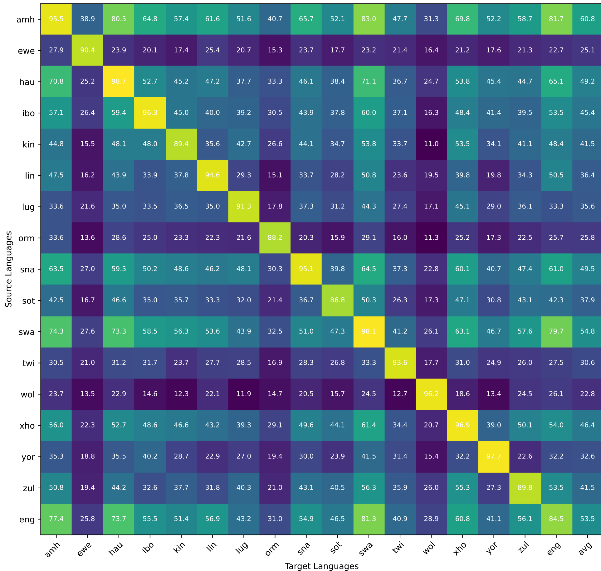
AfroXLMR-76L Intent Detection
