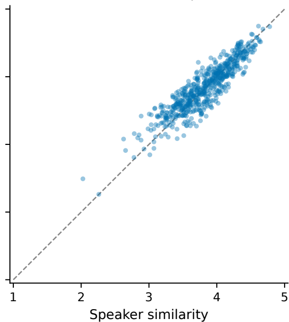
(b) Submitted weak-16 predictions
