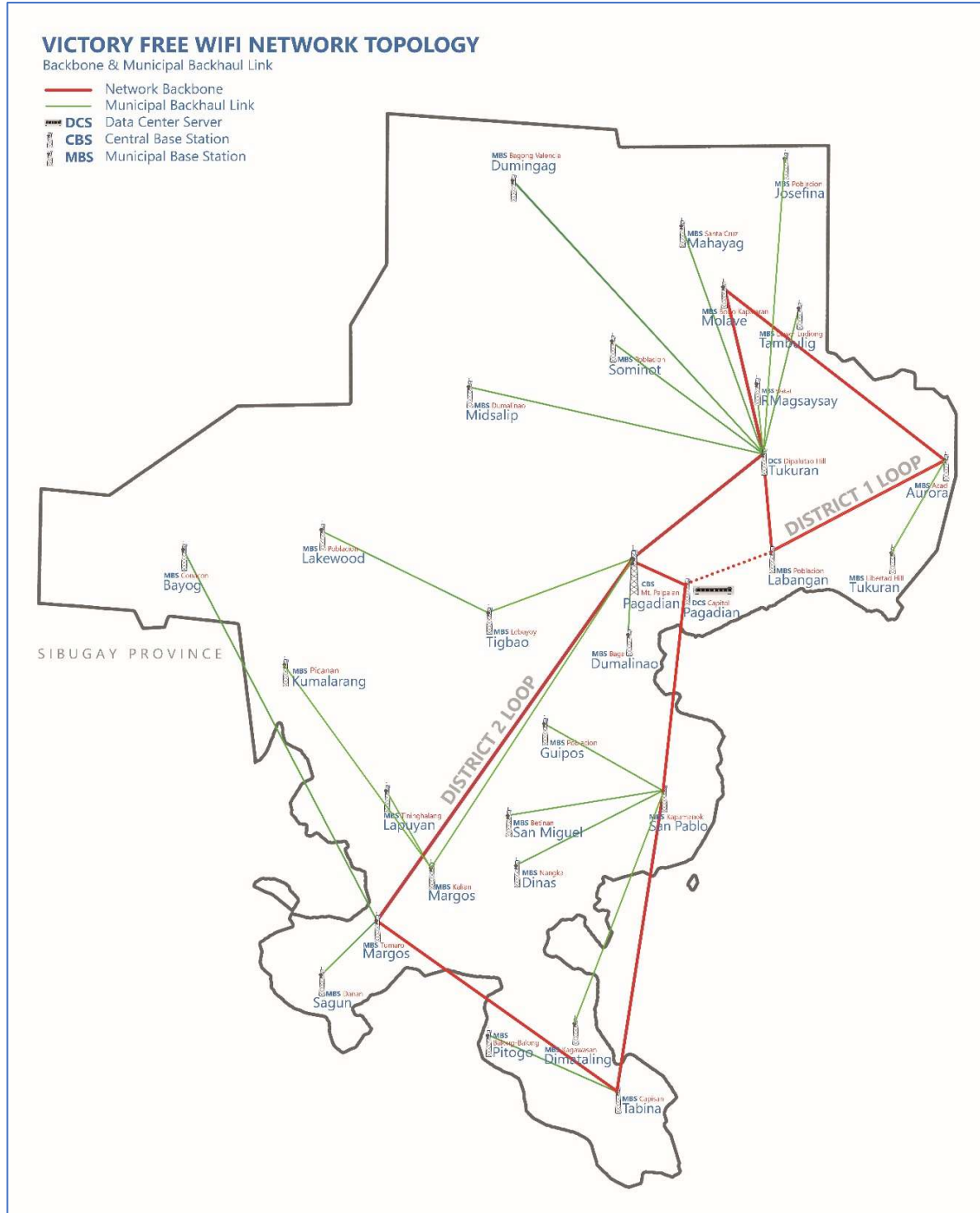
Fig 2. Network Backbone Link
