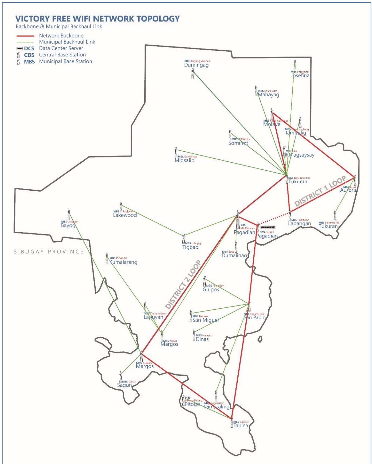
Figure 2. Network Backbone Links
