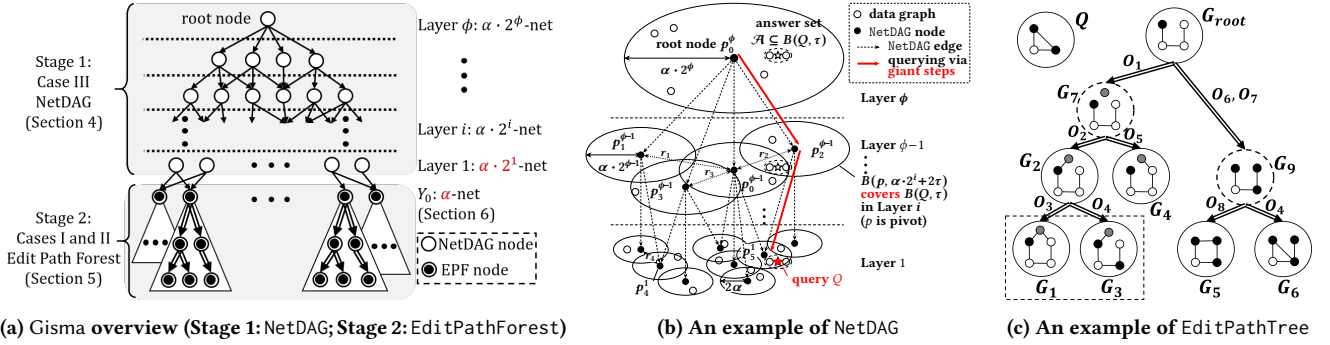
Figure 3: Overview of Gisma – Stage 1: NetDAG (Sec. 4); and Stage 2: EditPathForest (Sec. 5). Both indices depend on the threshold \alpha : the leaf layer of NetDAG is a 2\alpha -net, and \alpha is the radius of the balls indexed by EPTs.
