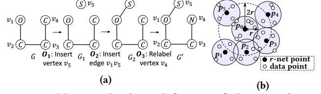
Figure 2: (a) A graph edit path [O_1, O_2, O_3] that transforms graph G into graph G' , resulting in a GED of 3; (b) An illustration of an r -net, where solid dots p_i , 0 \leq i \leq 5 are r -net centers, and small circles are data points in database \mathcal{D} .
