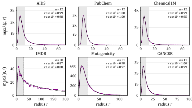
Figure 12: Two-stage fit for the six real datasets, on linear axes. Each curve is split at the threshold radius \alpha (grey dashed line, with the shaded band marking r \leq \alpha ) into a rising stage fitted by a skew-normal distribution and a tail stage fitted by an exponential decay G(\alpha) e^{-k(r-\alpha)} (both drawn as black dashed lines), which meet continuously at \alpha ; each panel reports the R^2 of the two stages, both fitted with p < 0.001 .
