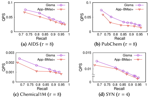
Figure 8: Comparison of QPS-recall curves
