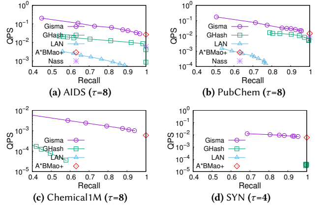
Figure 10: QPS-recall curves (log scale)
