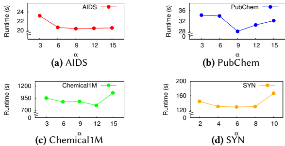
Figure 9: Effects of \alpha on runtime performance
