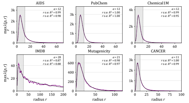
Figure 12: Two-stage fit for the six real datasets, on linear axes. Each curve is split at the threshold radius \alpha (grey dashed line, with the shaded band marking r \leq \alpha ). When r \leq \alpha , the curve is fitted by a skew-normal density; when r \geq \alpha , it is fitted by an exponential decay G(\alpha) e^{-k(r-\alpha)} (both drawn as black dashed lines). The two fits meet continuously at \alpha ; each panel reports their R^2 , with p < 0.001 for both.
