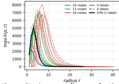
Figure 13: \max_p \lambda(p, r) versus radius r on the 18 synthetic datasets (coloured by node count; solid: 2 labels, dashed: 4 labels) together with the benchmark SYN dataset (the single-label case; thick black). Every curve shows the same two-stage shape, and the radius at the peak increases with graph size.
