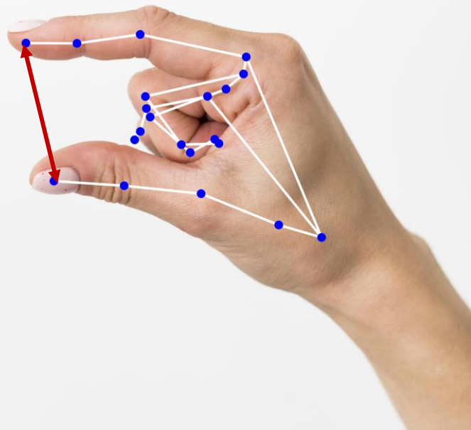
Thumb–index distance
