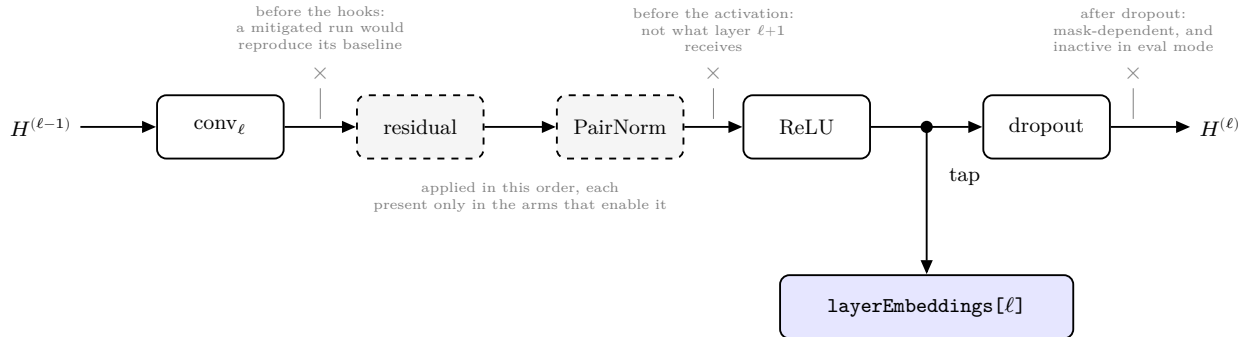
Figure 7: One layer’s interior and the point at which its representation is recorded. The tap sits after the convolution, after every mitigation hook, and after the activation, but before dropout. The three crossed positions are the alternatives this subsection rejects, each labeled with the reason. Hook boxes are dashed because a hook is present only in the arms that enable it; their order is fixed at residual before PairNorm regardless of the order in which the mitigation names are supplied.
