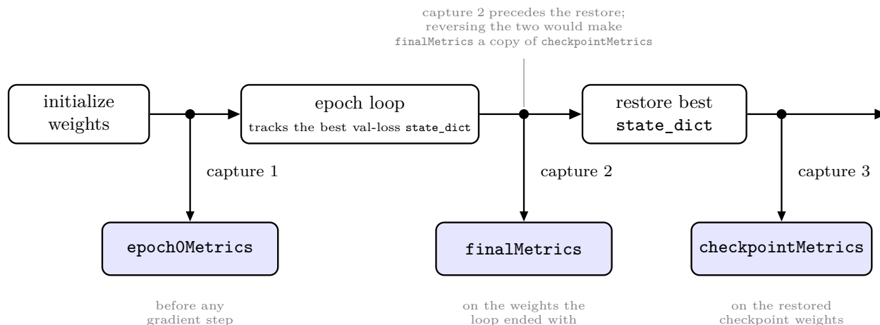
Figure 8: The order of the three metric captures within one run. Each is a separate eval-mode forward pass, never reused from a training-mode one. The capture on the final epoch’s weights is taken before the best-validation state_dict is restored, not after: taking it afterward would leave finalMetrics holding the same values as checkpointMetrics on every run, which would remove the only recorded difference between the weights a run ended with and the weights it is reported on.
