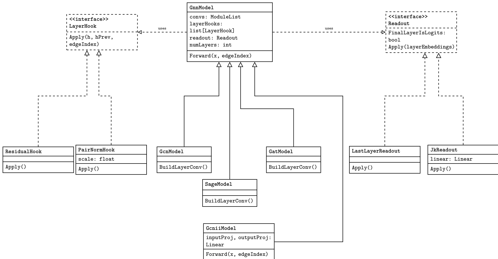
Figure 15: GnnModel and its four architecture subclasses (@sec-per-module-walkthroughs’s models entry), the LayerHook/Readout composition seam mitigations implements against (@sec-per-module-walkthroughs’s mitigations entry), and the two tested realizations of each protocol.
