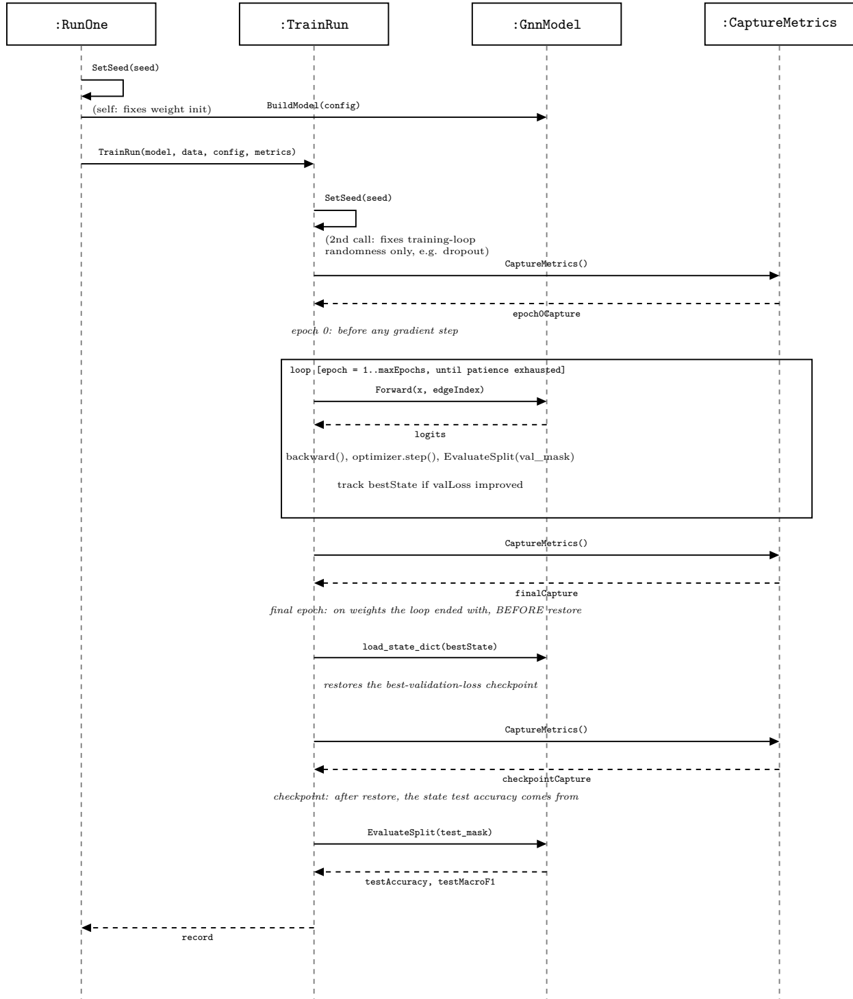
Figure 16: The call sequence for one run, from RunOne through the three metric captures ( @sec-three-metric-capture-points ), showing the two SetSeed calls ( @sec-per-module-walkthroughs's experiments entry) and that the final-epoch capture happens before, not after, the checkpoint restore ( @sec-training-and-evaluation-harness ).
