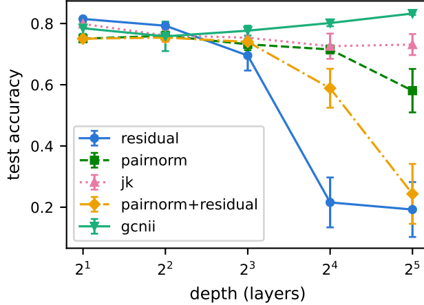
Figure 10: Test accuracy versus depth, GCN mitigation ablation (arm B) plus GCNII (arm C).
