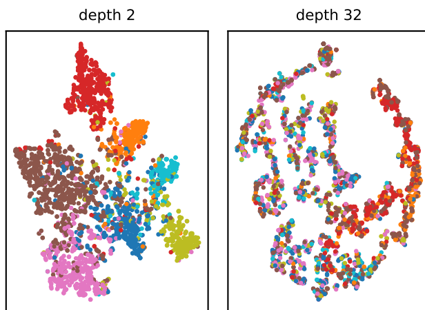
Figure 11: t-SNE projection of the checkpoint-capture layer embeddings, unmitigated GCN, seed 0, depth 2 versus depth 32, colored by class label. Fitted separately per panel; random_state=0 , perplexity=30 .
