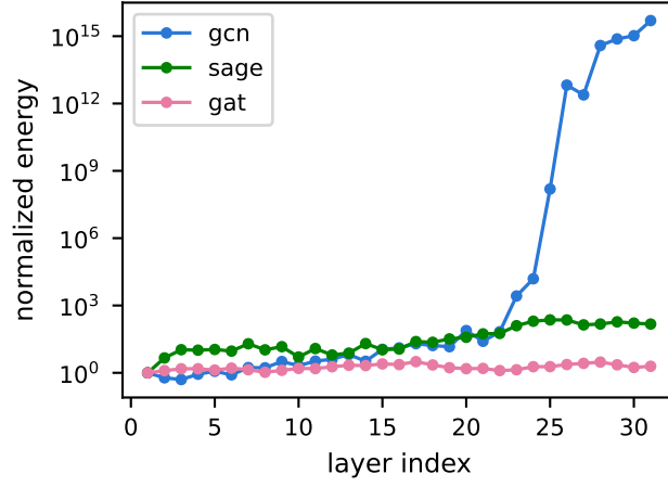
Figure 7: Normalized per-dimension energy versus layer index, checkpoint capture, depth 32, unmitigated GCN/GraphSAGE/GAT.
