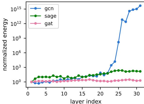
Figure 2: Normalized per-dimension energy versus layer index, checkpoint capture, depth 32, unmitigated GCN/GraphSAGE/GAT.
