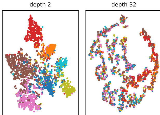
Figure 14: t-distributed stochastic neighbor embedding (t-SNE) (Maaten and Hinton 2008) projection of the checkpoint-capture layer embeddings, unmitigated GCN, seed 0, depth 2 versus depth 32, colored by class label. Fitted separately per panel; random_state=0 , perplexity=30 .
