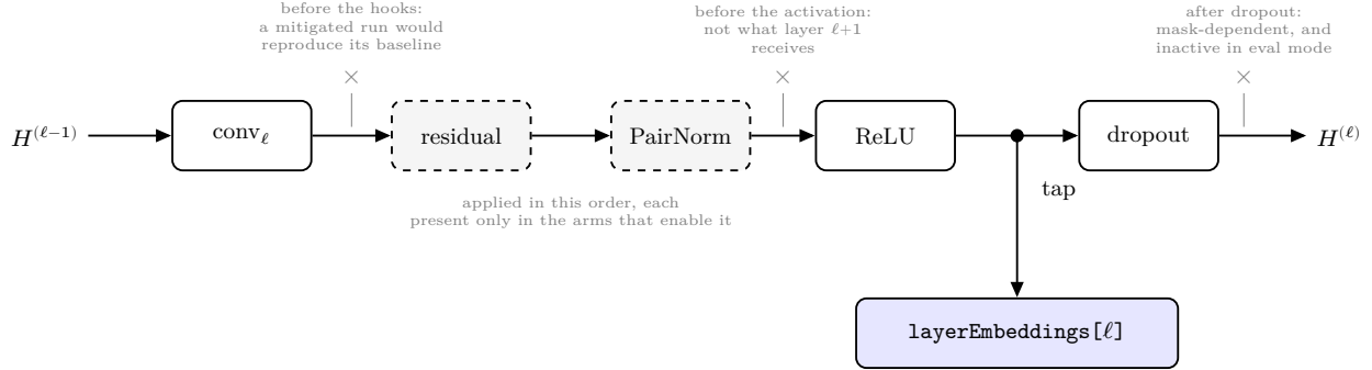
Figure 6: One layer’s interior and the point at which its representation is recorded. The tap sits after the convolution, after every mitigation hook, and after the activation, but before dropout. The three crossed positions are the alternatives this subsection rejects, each labeled with the reason. Hook boxes are dashed because a hook is present only in the arms that enable it; their order is fixed at residual before PairNorm regardless of the order in which the mitigation names are supplied.
