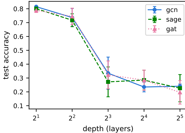
Figure 8: Test accuracy versus depth, unmitigated GCN, GraphSAGE, and GAT (arm A).
