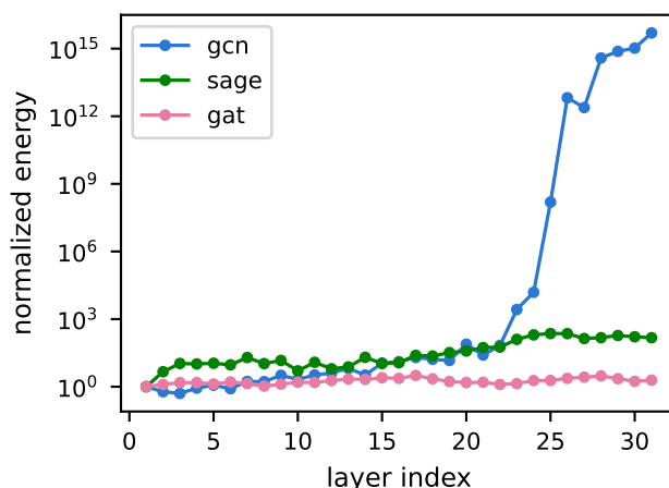
Figure 9: Normalized per-dimension energy versus layer index, checkpoint capture, depth 32, unmitigated GCN/GraphSAGE/GAT.
