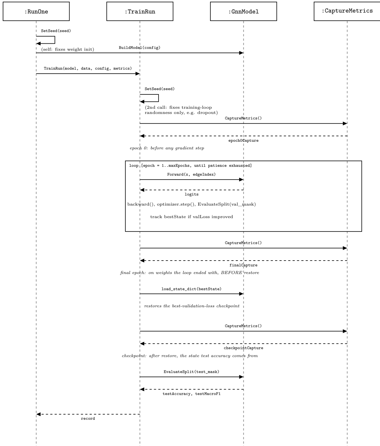
Figure 15: The call sequence for one run, from RunOne through the three metric captures ( @sec-three-metric-capture-points ), showing the two SetSeed calls ( @sec-per-module-walkthroughs's experiments entry) and that the final-epoch capture happens before, not after, the checkpoint restore ( @sec-training-and-evaluation-harness ).
