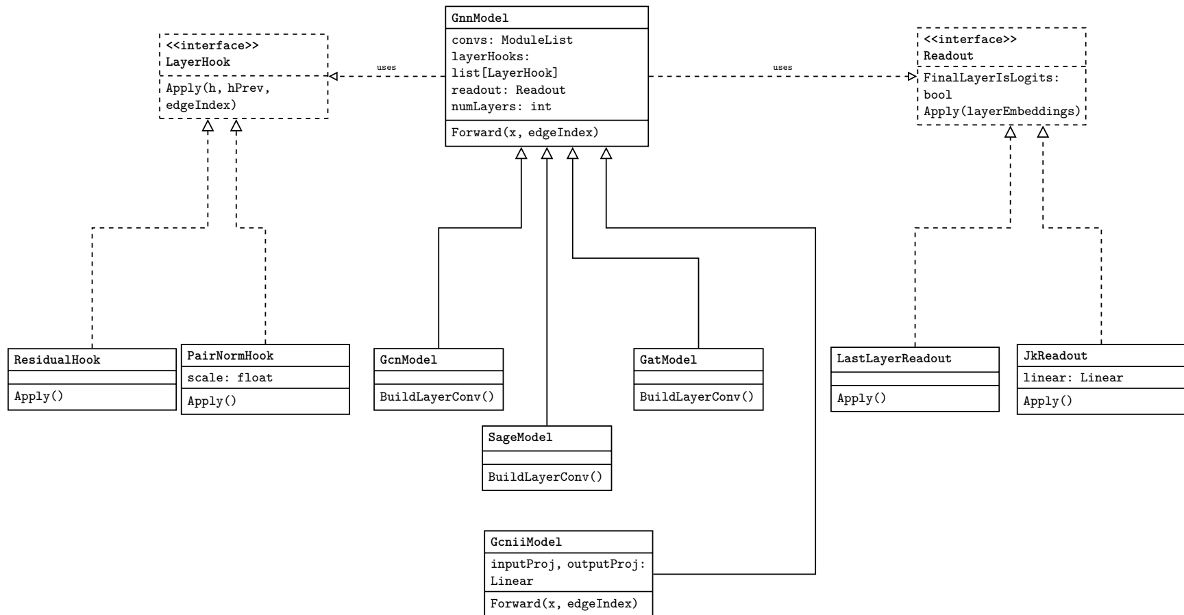
Figure 14: GnnModel and its four architecture subclasses (@sec-per-module-walkthroughs’s models entry), the LayerHook/Readout composition seam mitigations implements against (@sec-per-module-walkthroughs’s mitigations entry), and the two tested realizations of each protocol.
