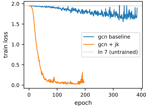
Figure 11: Training loss versus epoch, depth 32: unmitigated GCN baseline versus GCN with Jumping Knowledge.
