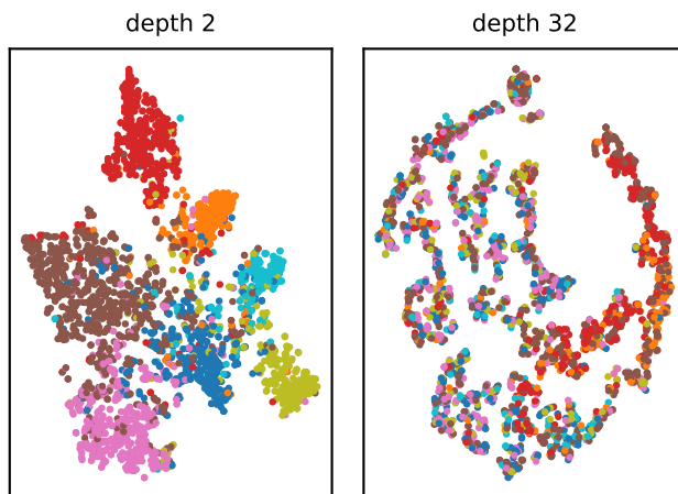
Figure 13: t-SNE projection of the checkpoint-capture layer embeddings, unmitigated GCN, seed 0, depth 2 versus depth 32, colored by class label. Fitted separately per panel; random_state=0 , perplexity=30 .
