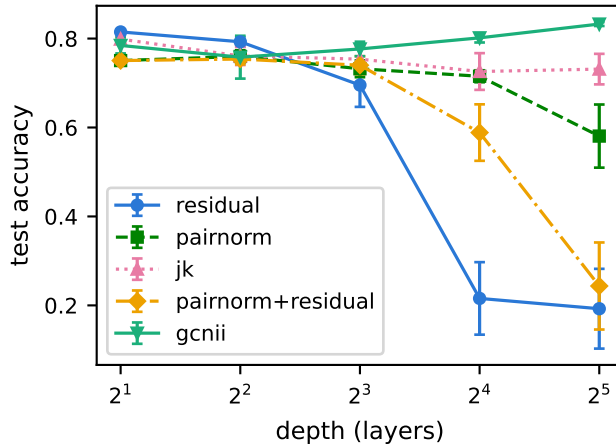
Figure 12: Test accuracy versus depth, GCN mitigation ablation (arm B) plus GCNII (arm C).
