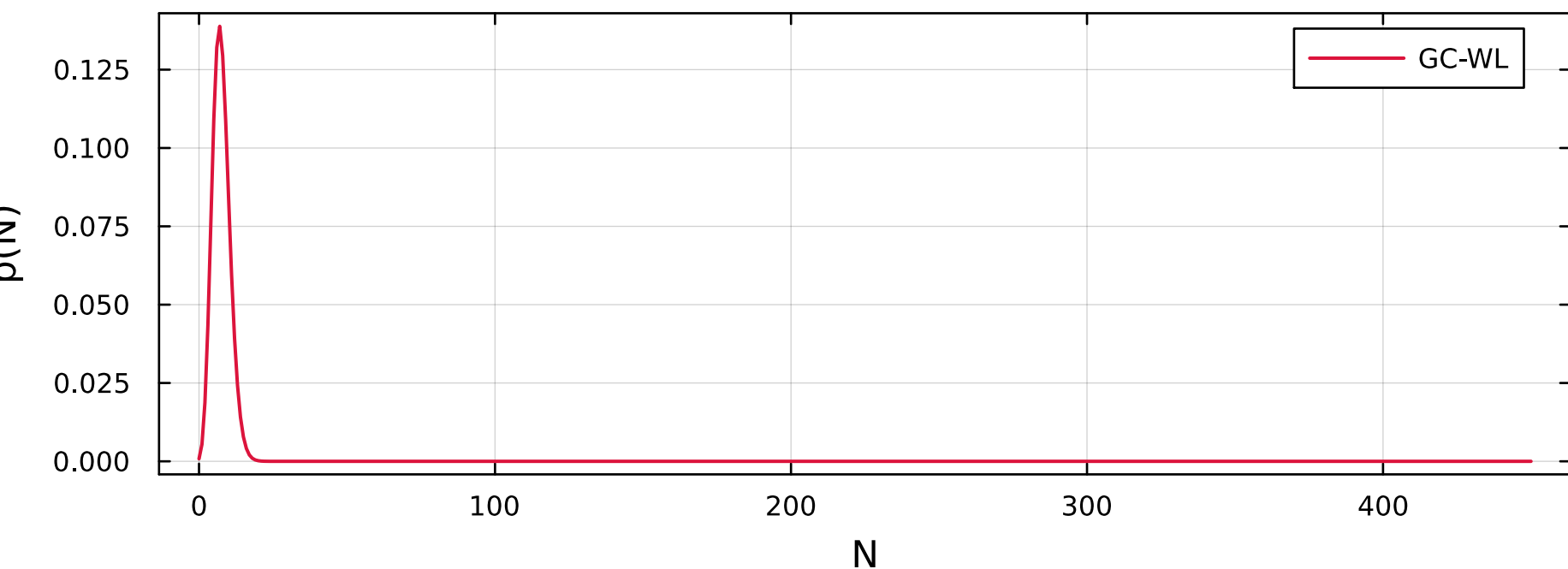
(c) Coexistence ( T = 140.46 K)
