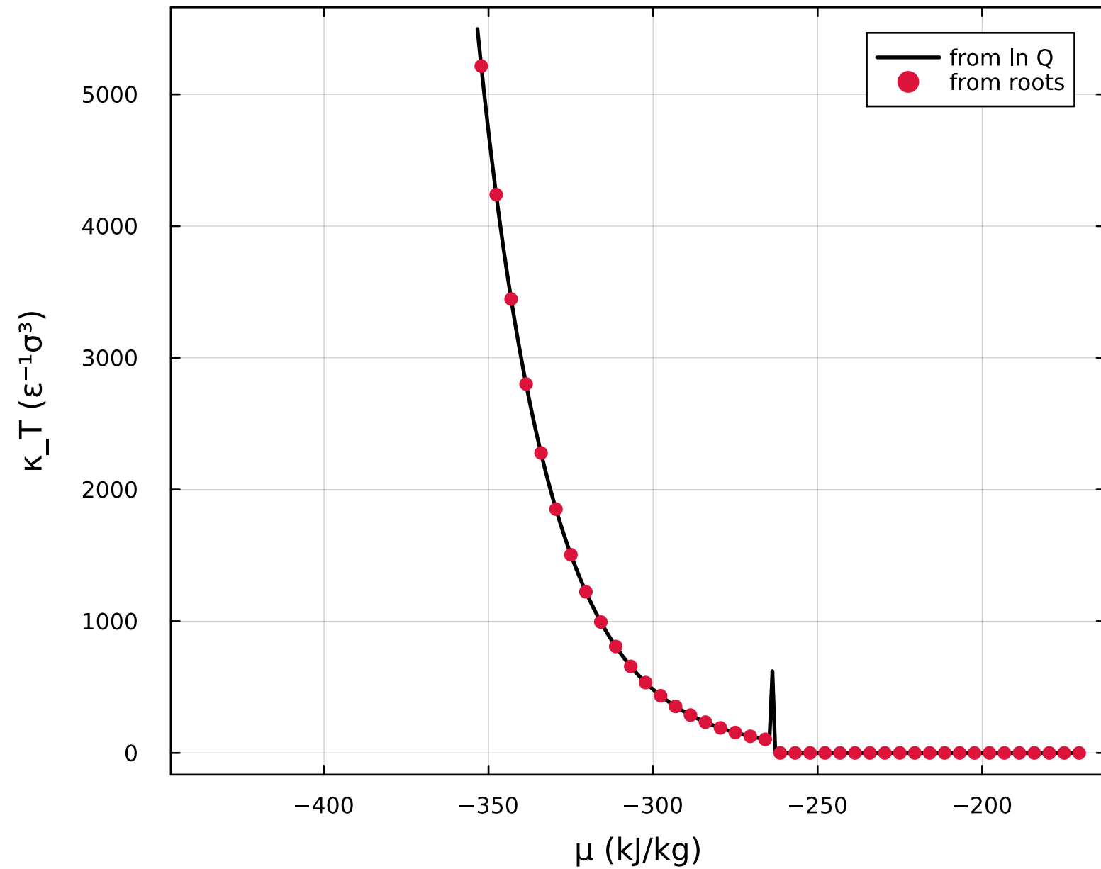
Compressibility \kappa_T(\mu) T^*=0.9
