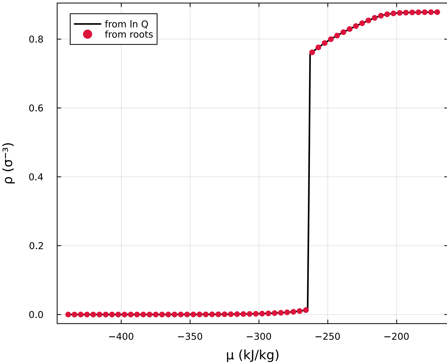
Density \rho(\mu) T^*=0.9
