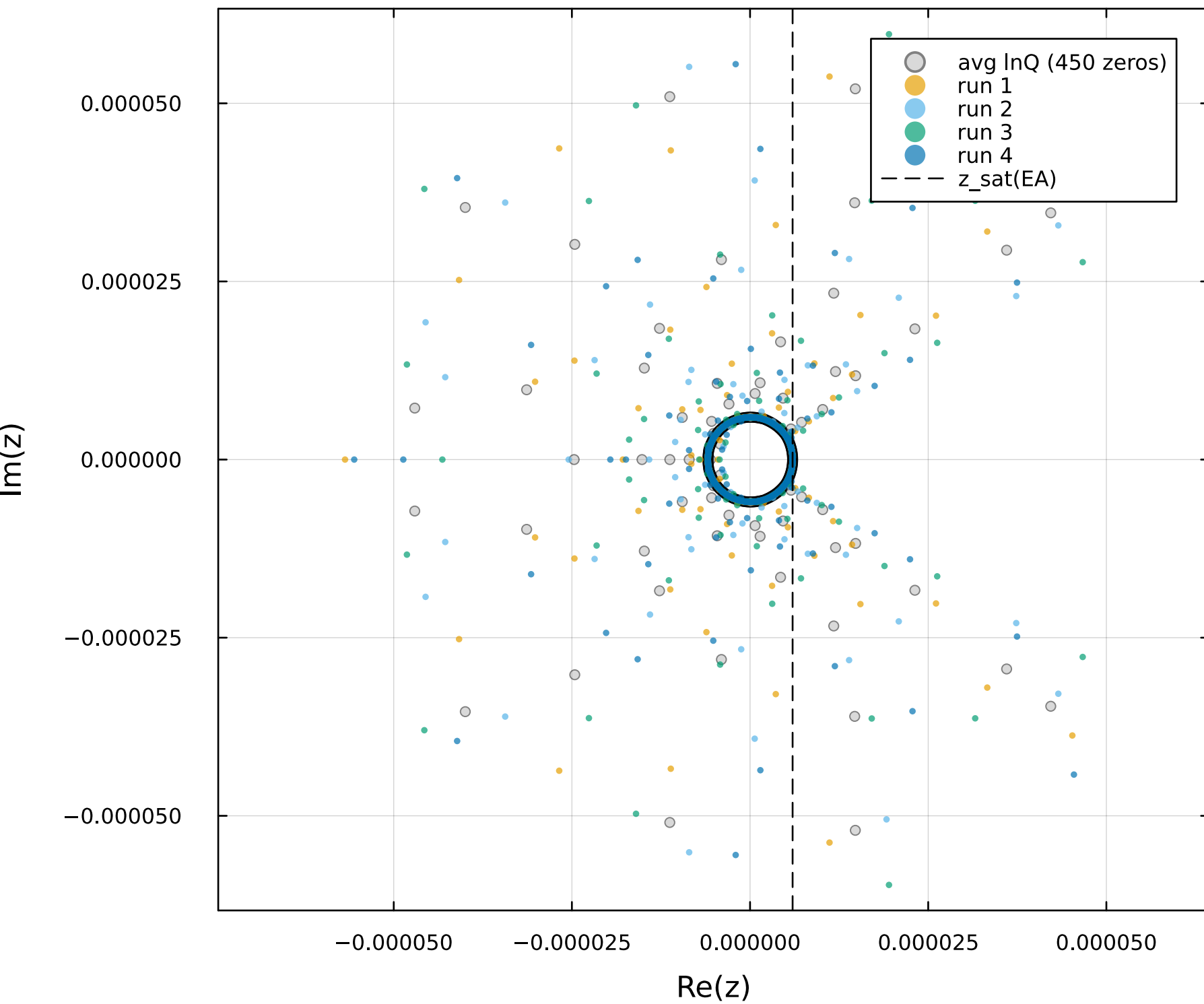
Yang-Lee zeros T^*=0.9 (all runs)
