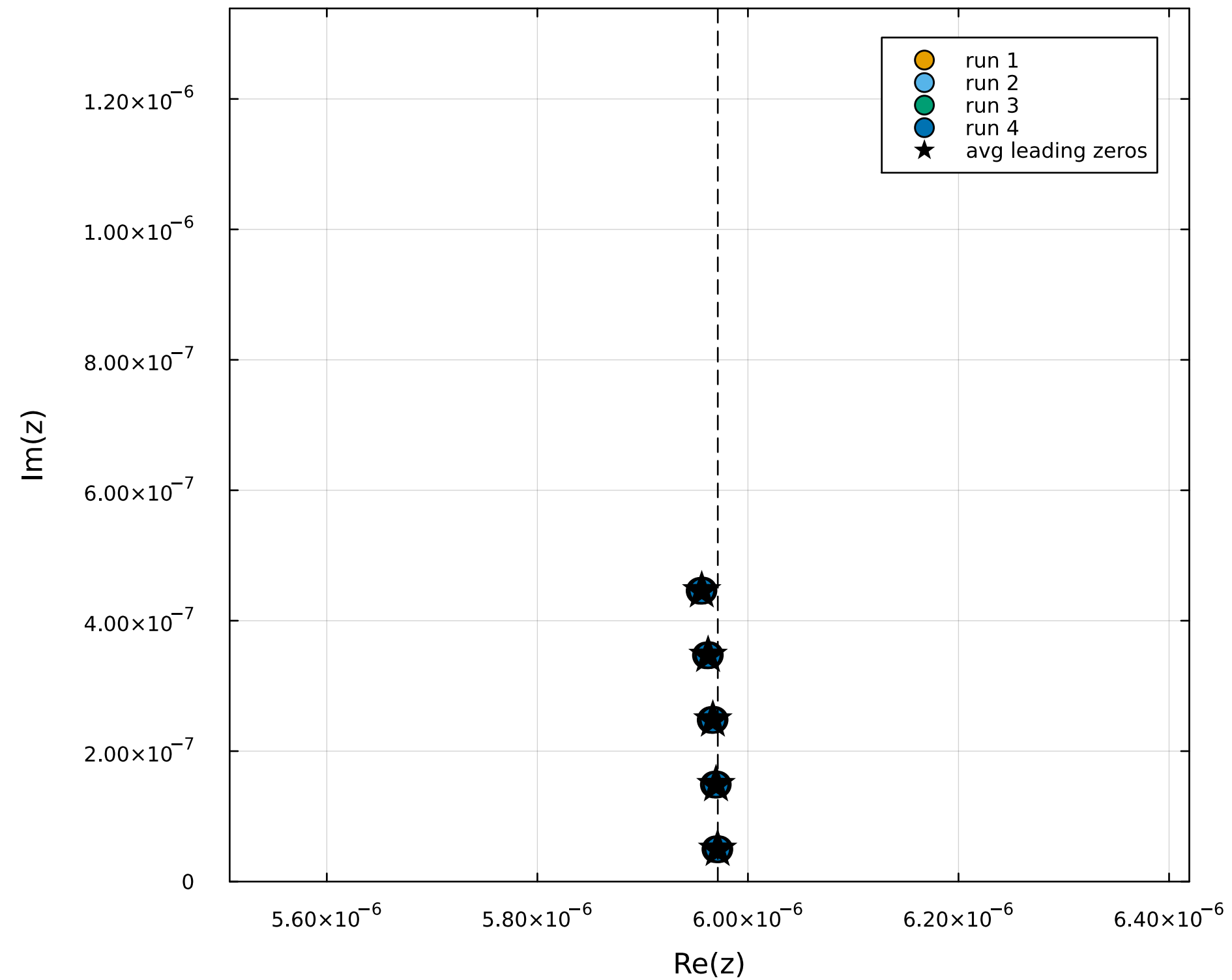
Leading Yang-Lee zeros (zoom)
