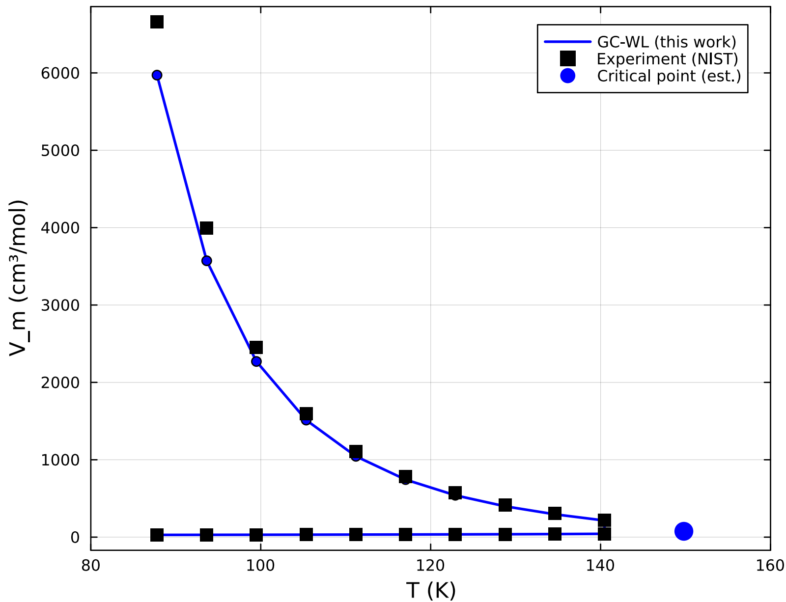
Argon: Vapor-Liquid Phase Diagram (V-T)
