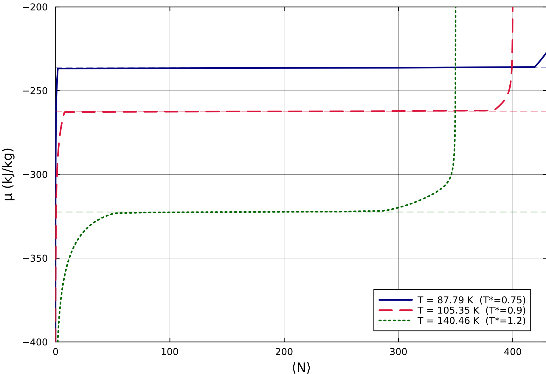
Chemical potential vs. average particle number
